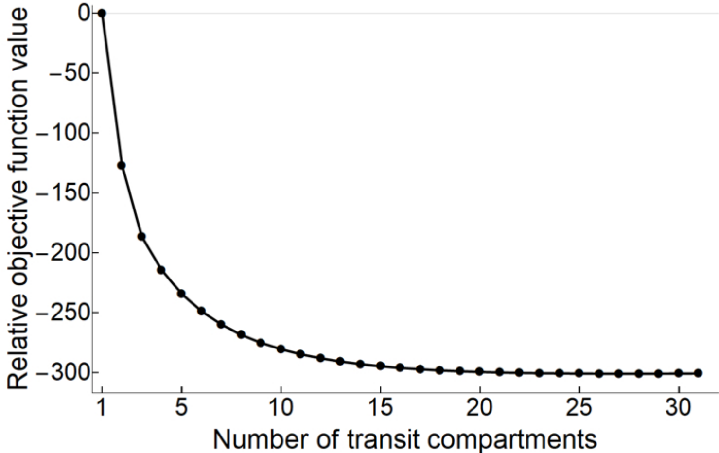
Objective function value vs. number of compartments
