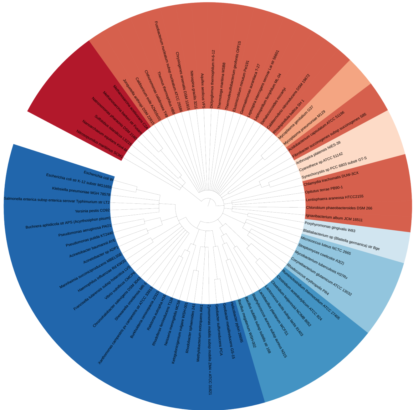
S2 Figure. Phylogenetic reference tree for species used in the analysis of conservation of essential genes (based on NCBI taxonomy).
