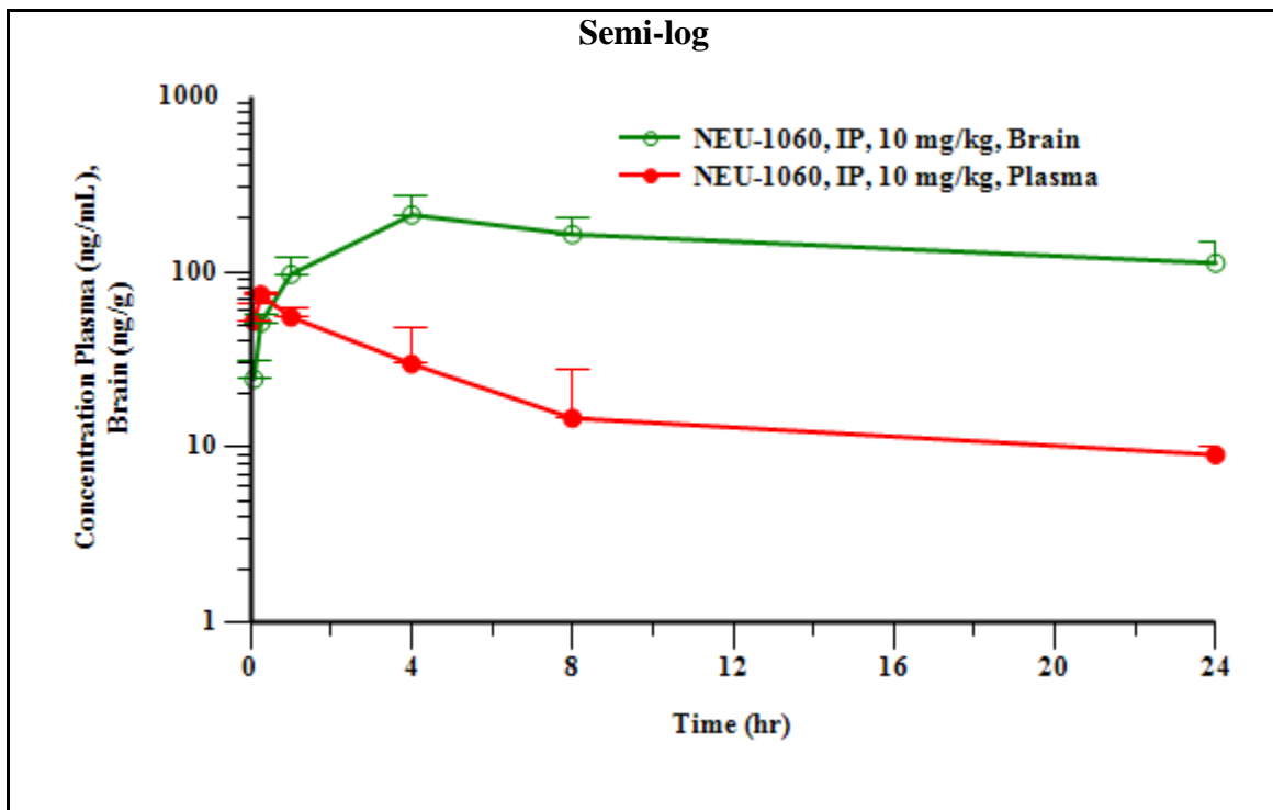
Figure S1. Mean plasma and brain concentration-time profiles of NEU-1060 (compound 14) following a single intraperitoneal administration in female BALB/c mice (Dose: 10 mg/kg)
