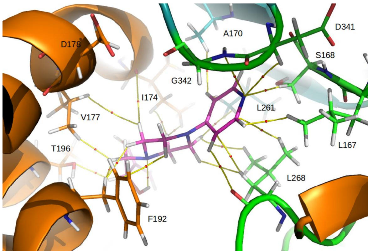
S2: Charge density molecular graph for the complex of SphK1 with compound 3 (in magenta). Yellow lines connecting the nuclei are the bond paths, and the small red spheres on them are the bond critical points (BCPs).
