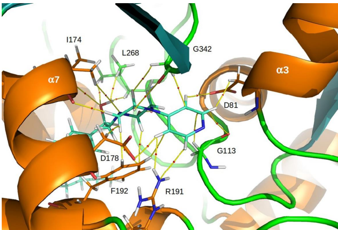
S1: Charge density molecular graph for the complex of SphK1 with compound 4 (in cyan). Yellow lines connecting the nuclei are the bond paths, and the small red spheres on them are the bond critical points (BCPs).
