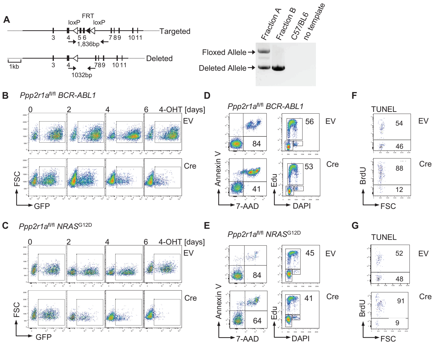
Figure S1: Effects of PP2A ablation on survival in B-cell lineage leukemia, Related to Figure 1.
