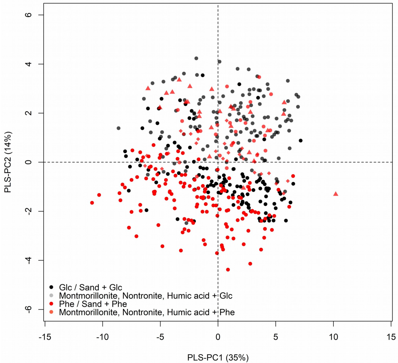
Figure S4. Partial Least Square Discriminant analysis (PLS-DA). Scores plot of the model calibrated to discriminate the C-source (phenanthrene (Phe) and glucose (Glc)) based on FTIR spectra.
