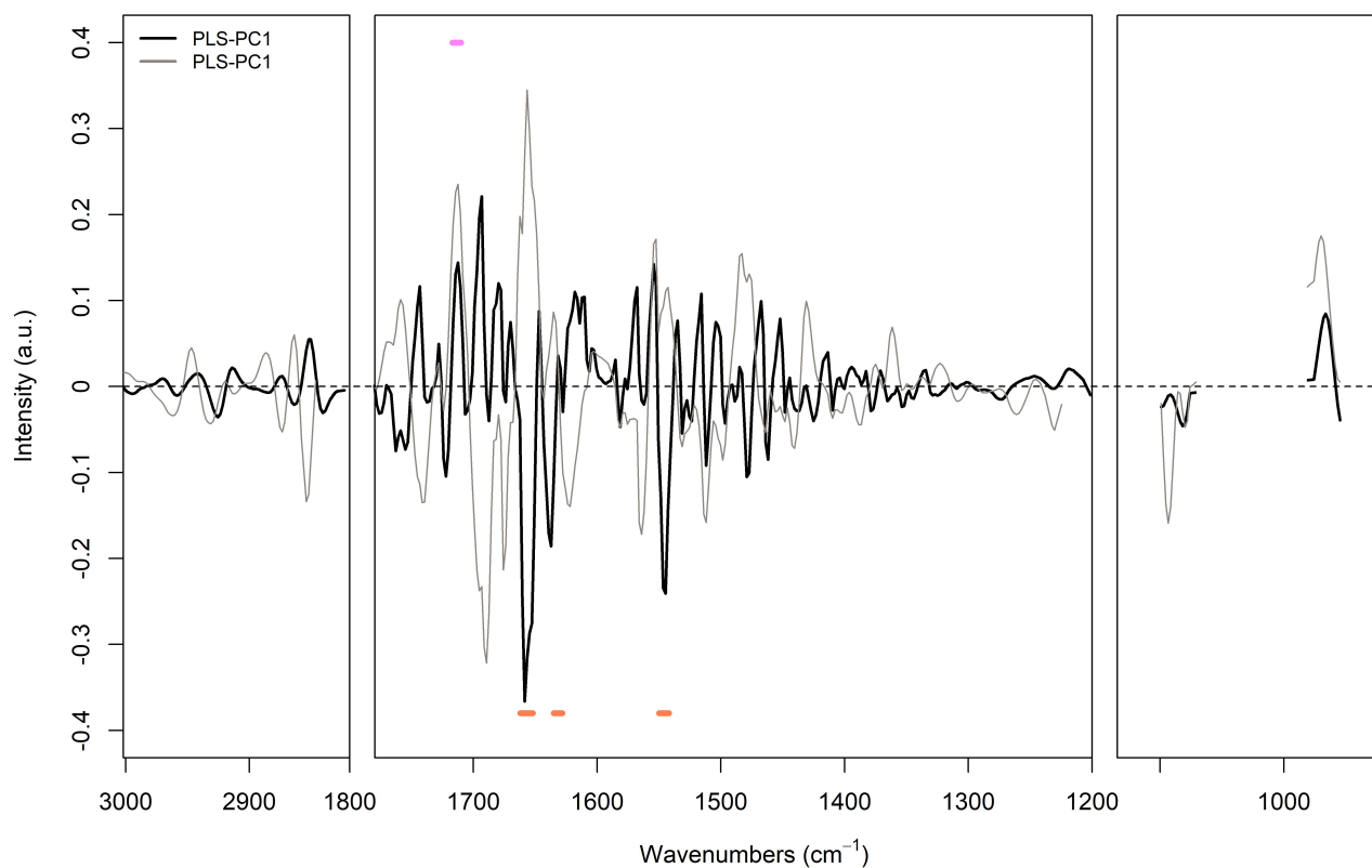
Figure S5. Loadings plot of the model discriminating for the C-source (glucose vs. phenanthrene) based on FTIR spectra. Horizontal bold lines in the loading plots represent the macromolecular assignment of the peaks (— proteins, — nucleic acids). The sign (-/+) of the bold lines reflect that of the corresponding loading of the PLS-PC1.
