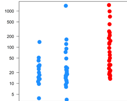
PF3D7_1036300
