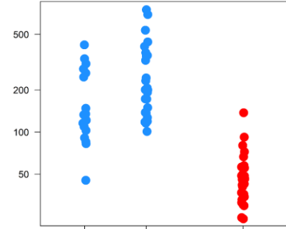
PF3D7_1327300
