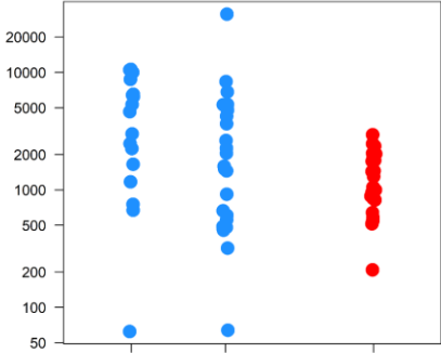
PF3D7_1302100
