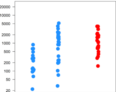
PF3D7_1302100
