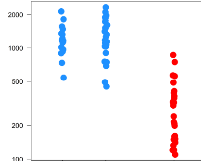
PF3D7_1036300
