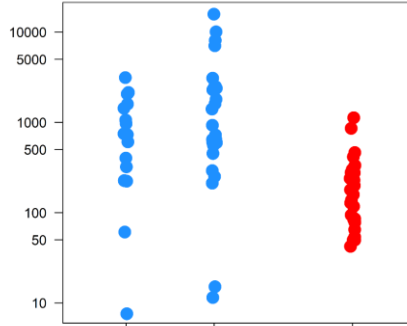
PF3D7_1030200
