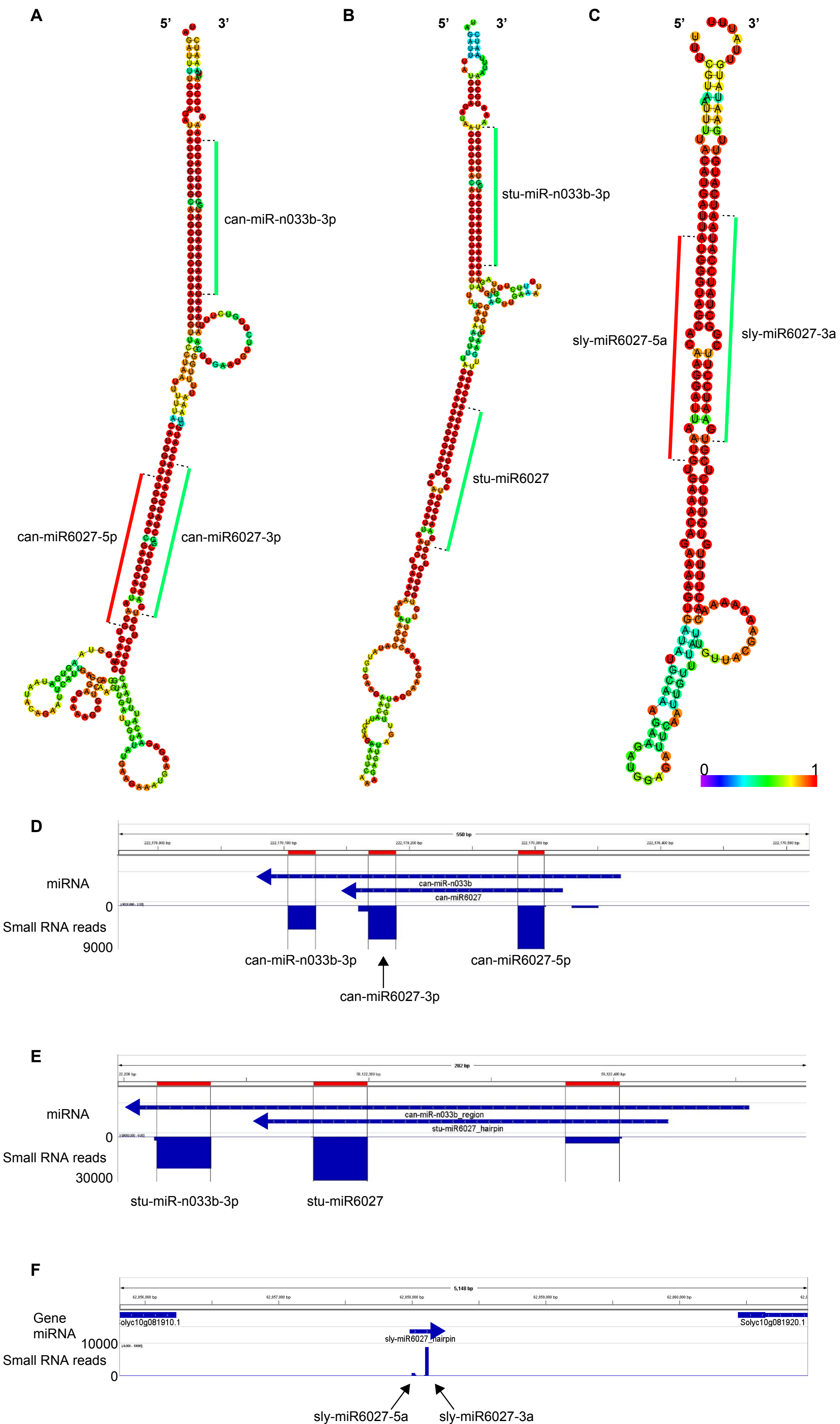
Figure S8. The hairpin structures of miR-n033b and their expression
