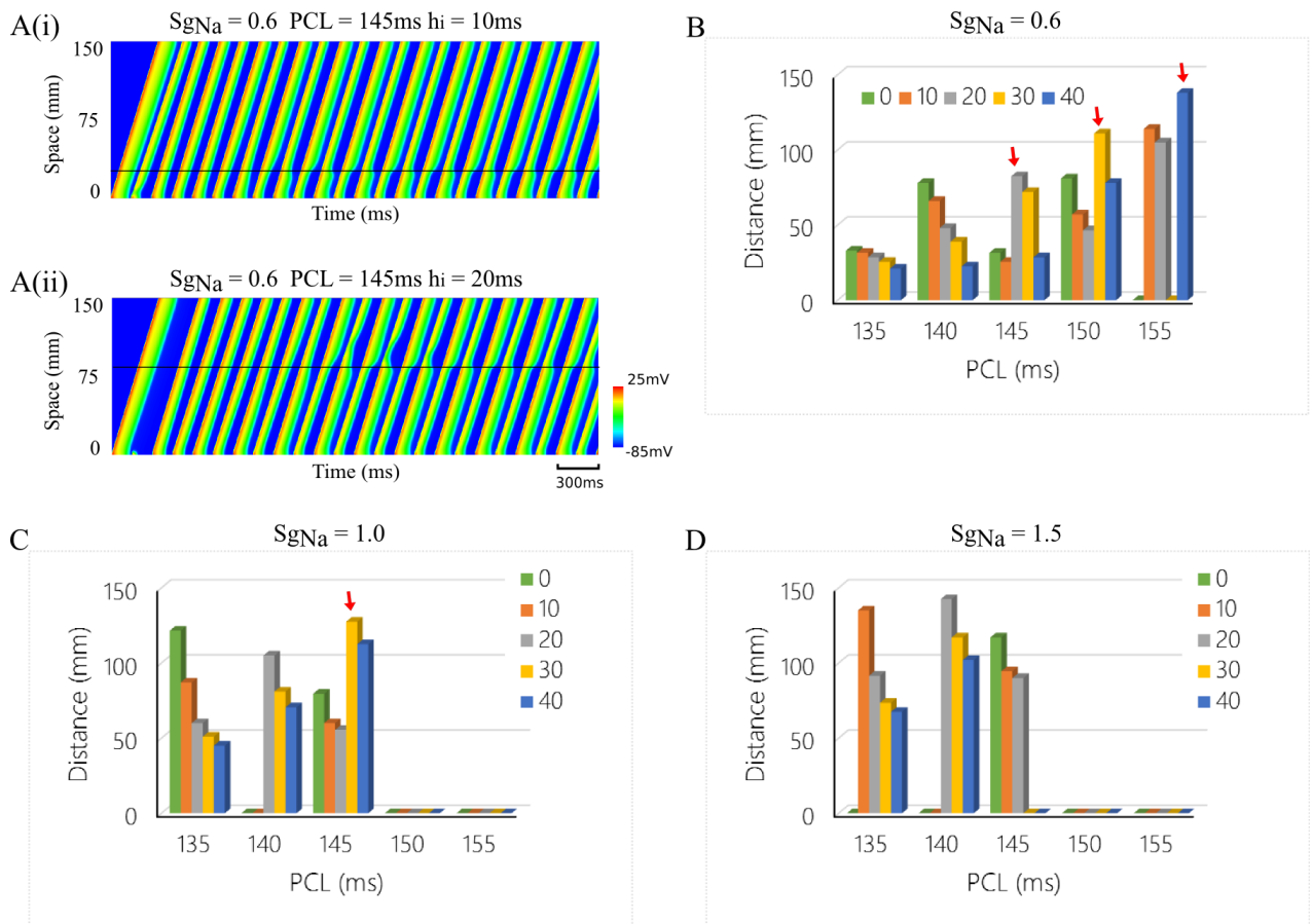
Fig S4 Role of I_{Na} recovery time in the location of APD node. (A) Representative 1D space-time results with S_{gNa}=0.6 , PCL = 145ms, h_i=10 ms (i) and 20ms (ii). (B) Statistic APD node distances from stimulation site at different recovery time prolongations and PCLs with reduced I_{Na} . (C) Statistic APD node distances from stimulation site at different recovery time prolongations and PCLs with normal I_{Na} . (D) Statistic APD node distances from stimulation site at different recovery time prolongations and PCLs with increased I_{Na} . Red arrow marked the APD node relocated conditions.
