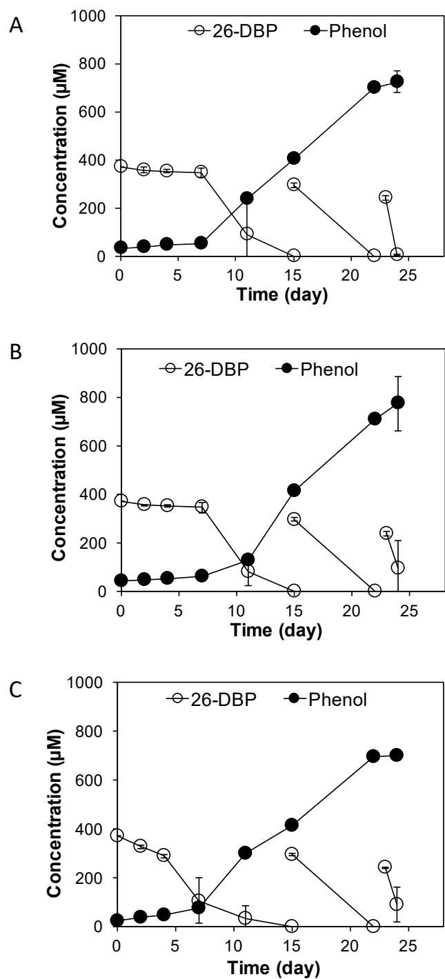
Figure S2. Debromination of 2,6-DBP and accumulation of phenol in Halodesulfovibrio marinesediminis (A), Desulfuromusa kysingii (B) and Desulfovibrio bizertensis (C) culture. The cultures were collected for an end point protein assay.
