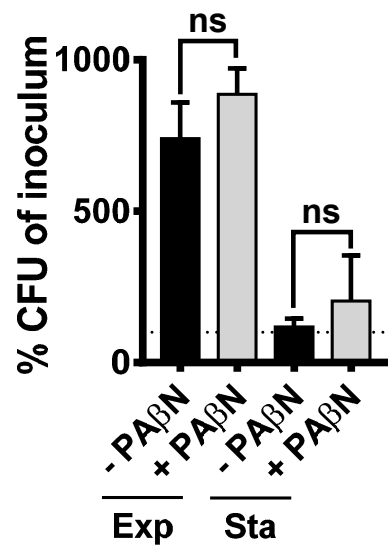
Figure S4. The efflux pump inhibitor phenylalanine-arginine \beta -naphthylamide (PA \beta N) does not affect bacterial viability. Colony forming units of K. pneumoniae harvested at exponential (Exp) or stationary (Sta) phase and incubated for 4 hr in medium containing the efflux pump inhibitor phenylalanine-arginine \beta -naphthylamide (PA \beta N, 40 \mu g/mL ) alone. Dotted horizontal line represents the number of colony forming units (CFU) prior to incubation. Error bars represent the standard deviation. A student's t-test was used to calculate statistical significance. ns not significant.
