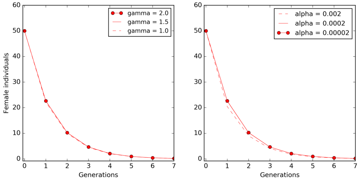
Figure S1. Model simulation of the IIT 1 experiment showing how the outcome of the population dynamics is influenced by the variation of \gamma and \alpha parameters.
