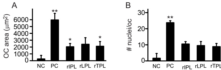
Supplemental Figure 3. RAW 264.7 cells were primed with RANKL (50 ng/mL) for 2 days and then cultured for an additional two days without RANKL treatment (negative control, NC), with RANKL (50 ng/mL, positive control, PC), with human recombinant plastin-1 (rIPL), 2 (rLPL) and 3 (rTPL) at 10 μg/mL. A) Average osteoclast planar area. B) Average number of nuclei per osteoclast. Data are means ± SEM, N= 30-55 cells, *p<0.05, **p<0.01 compared to NC assessed by student's t-test.
