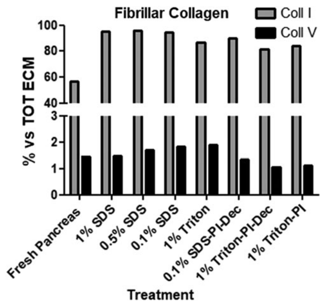
SUPPLEMENTARY FIG. S2. Quantitative proteomic analysis of the decellularized pECM hydrogels and fresh pancreas. Fibrillar collagen proteins.
