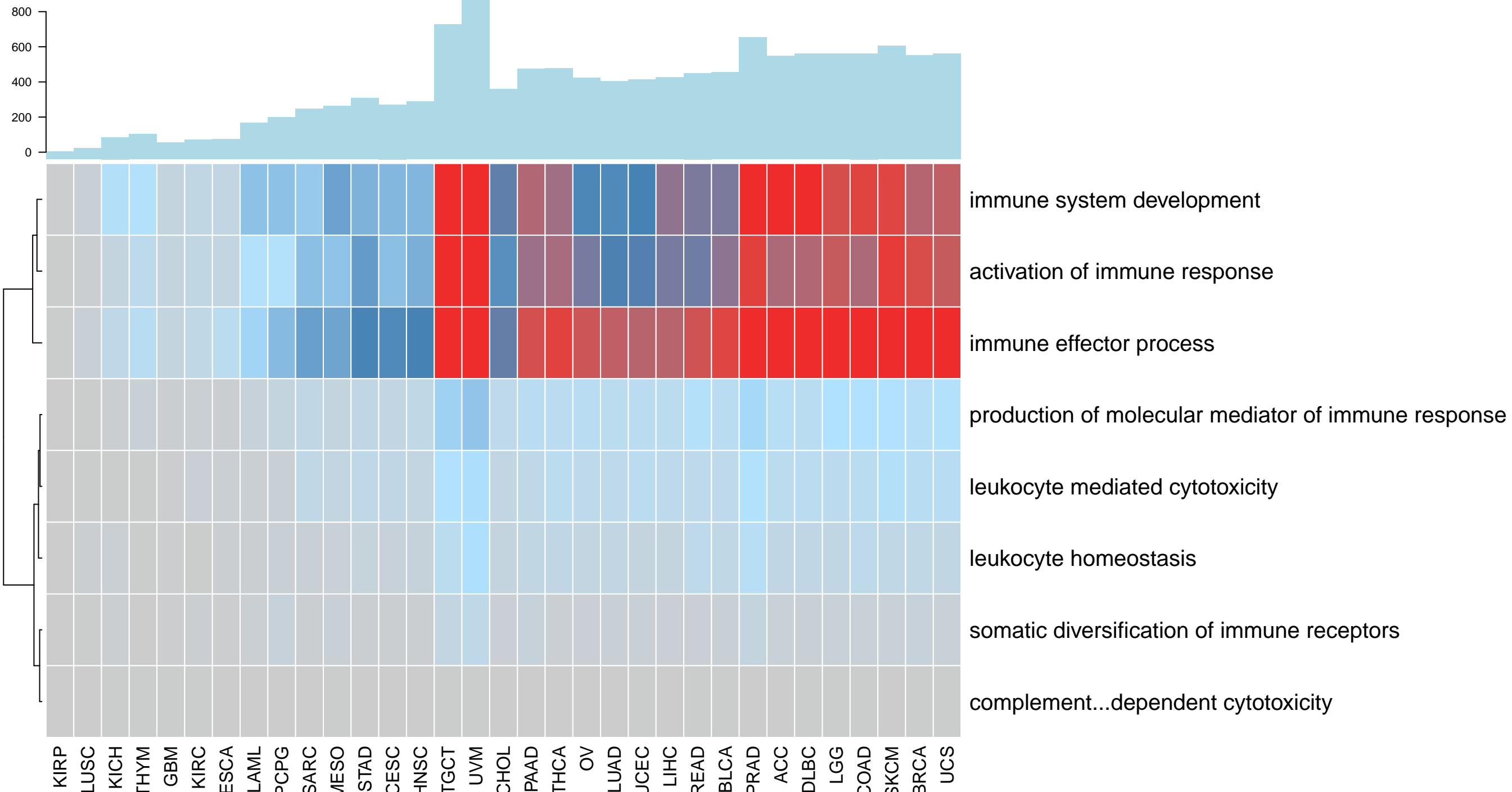
number of immune pathway genes
