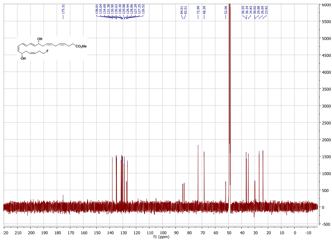
Figure S12 ^{13}\text{C-NMR} spectrum of 22-F-PD1-ME (4).
