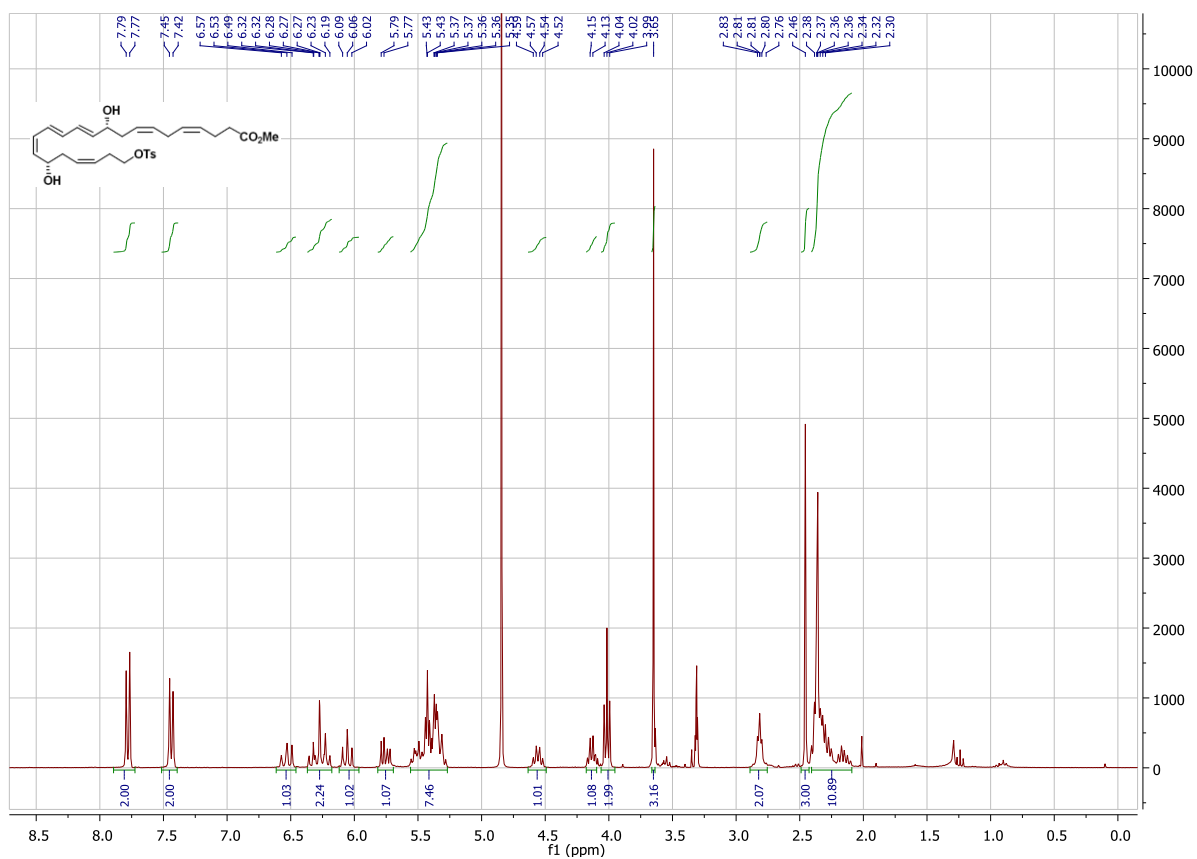
Figure S7 ^1\text{H-NMR} spectrum of methyl ester 12 .
