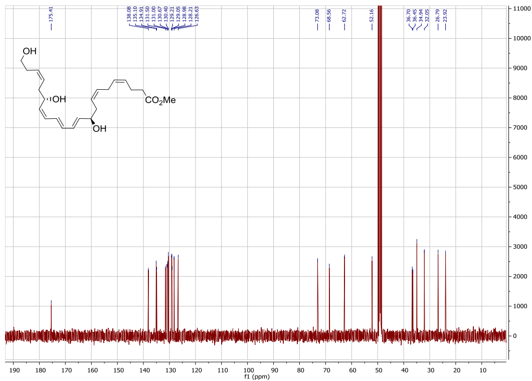
Figure S10 ^{13}\text{C-NMR} spectrum of methyl ester 11 . See reference 4 for comparison.
