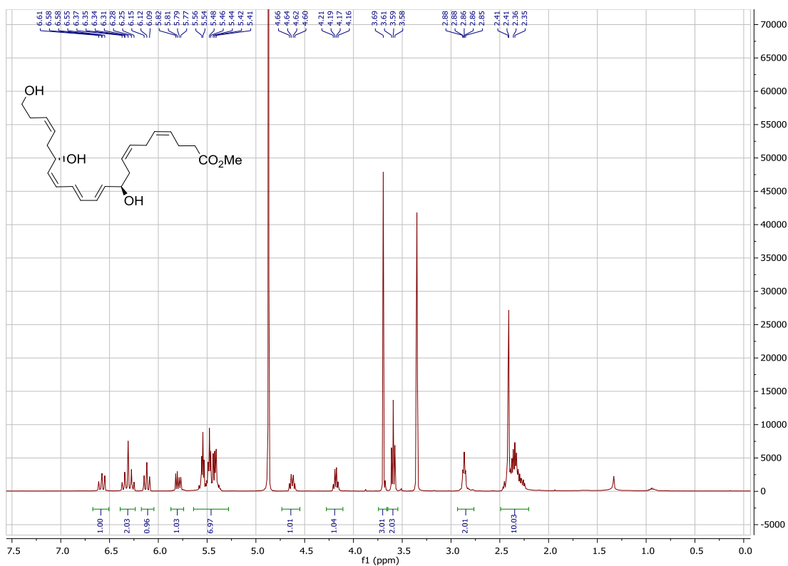
Figure S9 ^1\text{H-NMR} spectrum of methyl ester 11 . See reference 4 for comparison.
