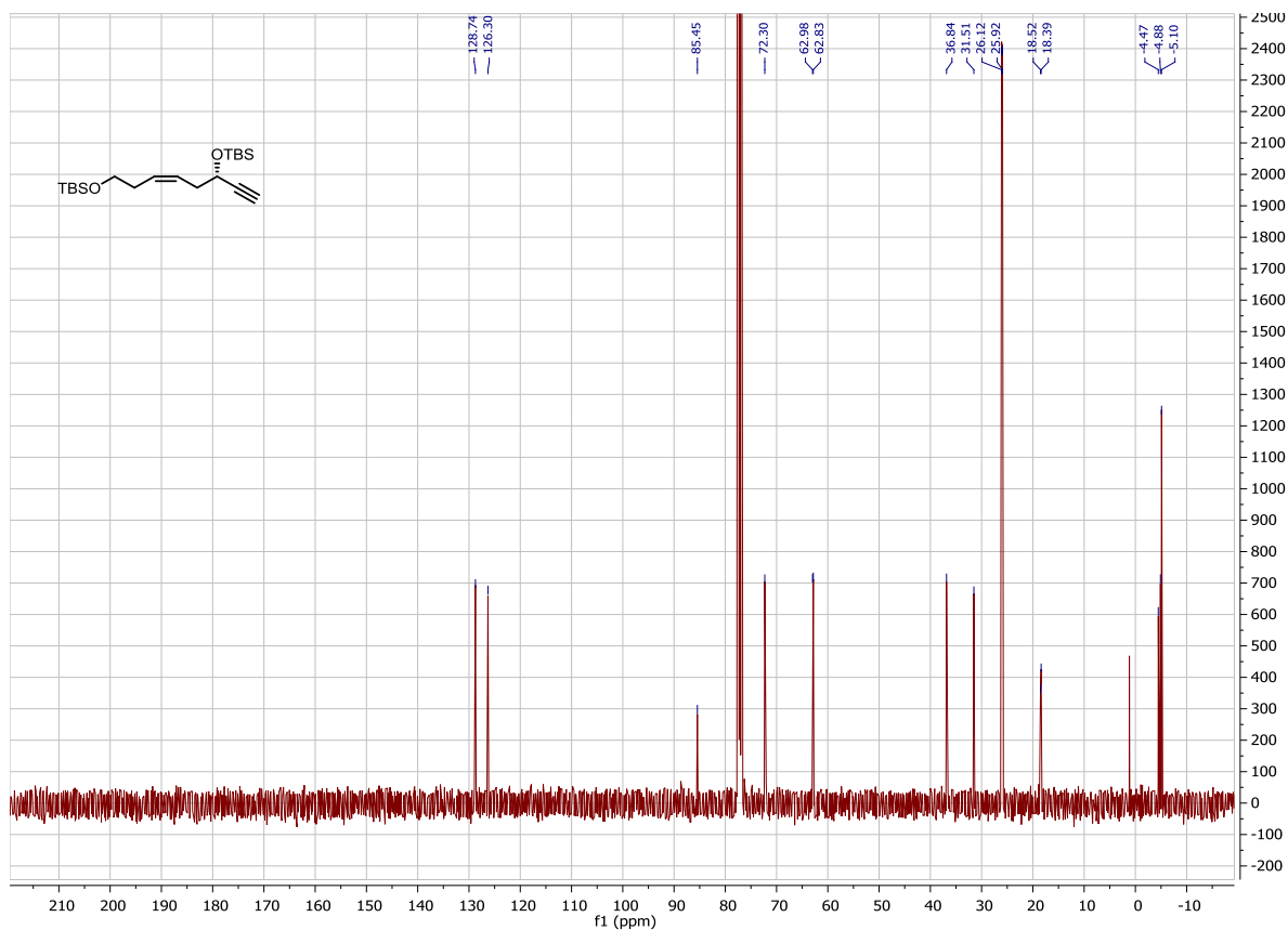
Figure S4 ^{13}\text{C-NMR} spectrum of 8 .
