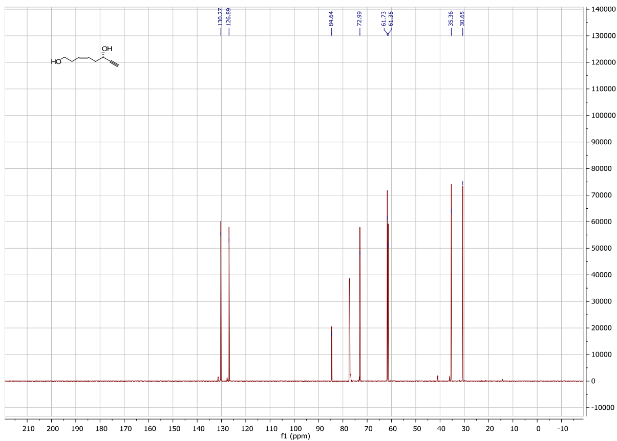
Figure S6 ^{13}\text{C} -NMR spectrum of 9.
