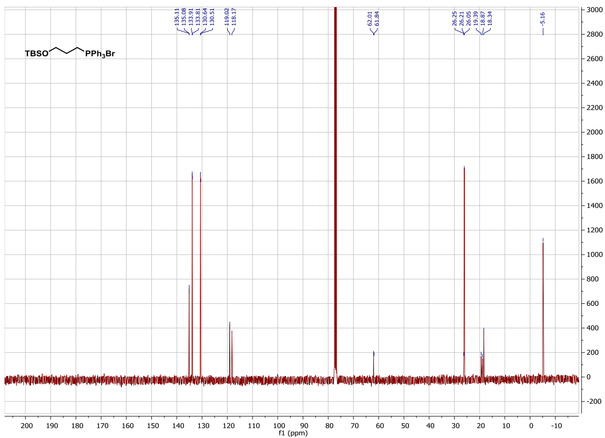
Figure S2 ^{13}\text{C-NMR} spectrum of 6 .
