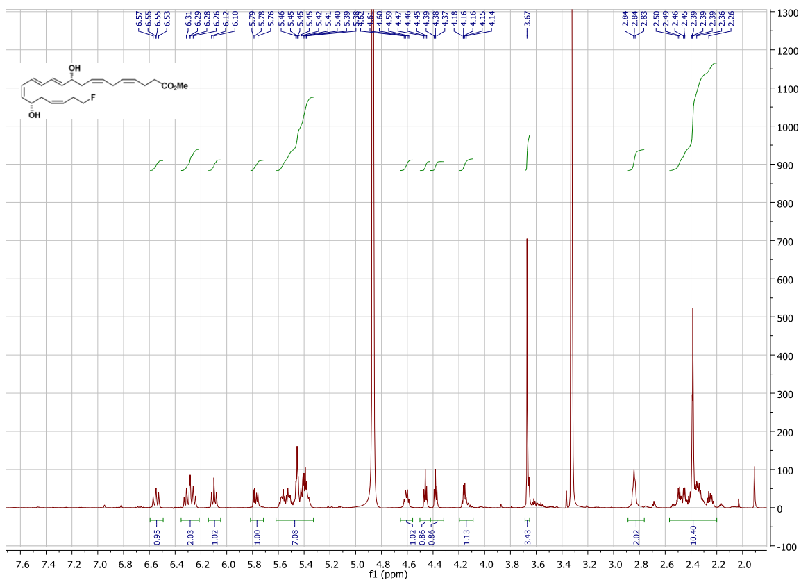
Figure S11 ^1\text{H-NMR} spectrum of 22-F-PD1-ME (4).
