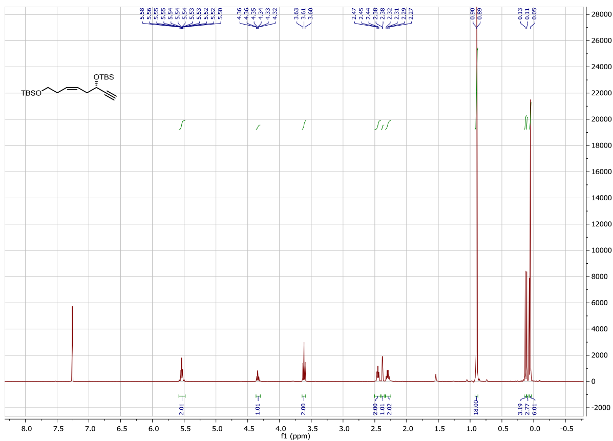
Figure S3 ^1\text{H-NMR} spectrum of 8 .
