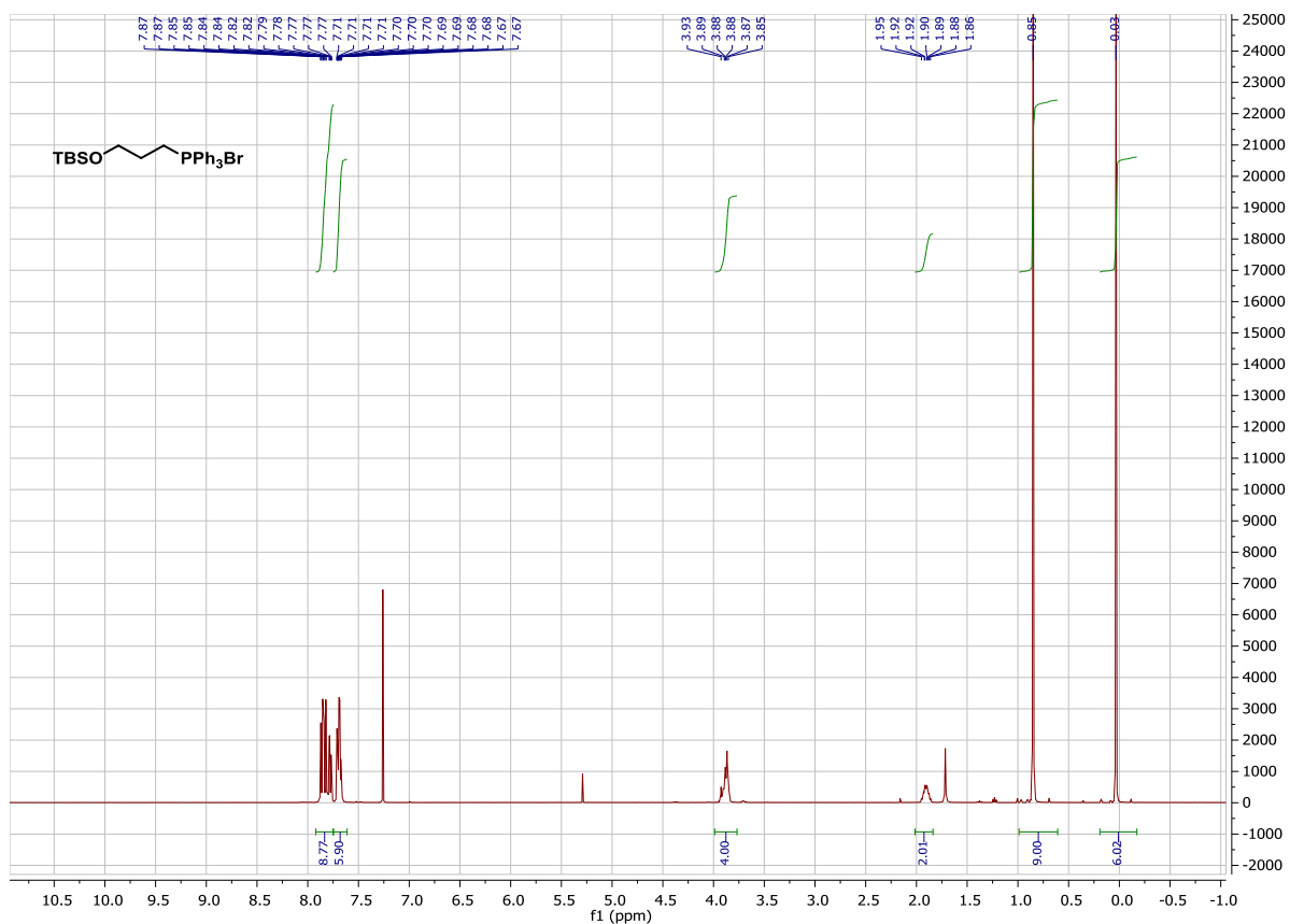
Figure S1 ^1\text{H-NMR} spectrum of 6 .
