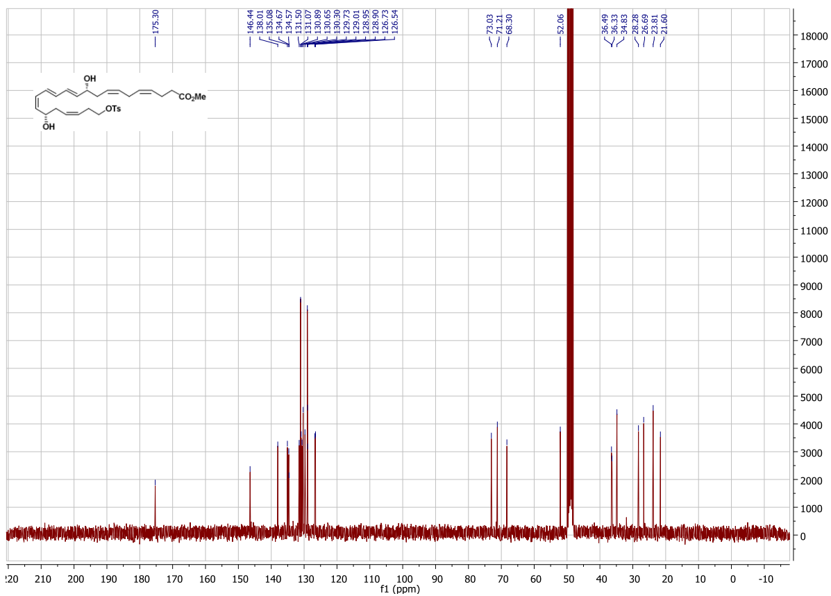
Figure S8 ^{13}\text{C-NMR} spectrum of methyl ester 12 .
