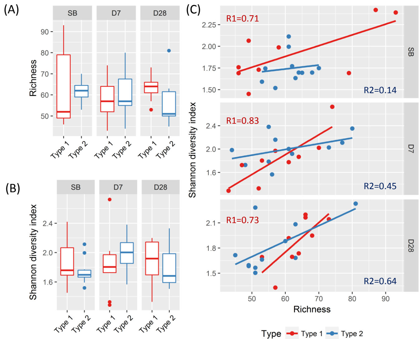
Figure S1. The differences of microbial diversity between the type 1 and 2 groups. (A) Boxplot of richness. In D28 samples, Type 1 and Type 2 differ significantly (p-value: 0.025). (B) Boxplot of Shannon diversity index. There is no statistical difference between the two types at each of the three collection times. (C) Correlation plots of richness and Shannon diversity index for each type at each collection time. The correlation coefficient between richness and Shannon diversity index of each type became closer from SB to D28.
