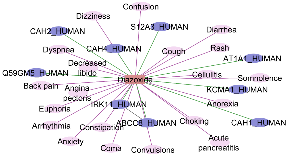
S7 Figure. Network of interactions between diazoxide and protein targets active in the metabolism of the human body, as well as the relationship with side effects.
