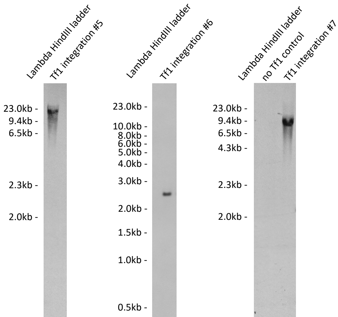
Supplemental Figure S5: Southern blot for the presence of Tf1-neo. The probe was located in the neo resistance gene of Tf1. Genomic DNA were digested with SphI for integrations #5 and #7, and with BstXI for integration #6. Expected sizes were 11.4kb for integration #5, 2.5kb for integration #6 and 8.7kb for integration #7.
