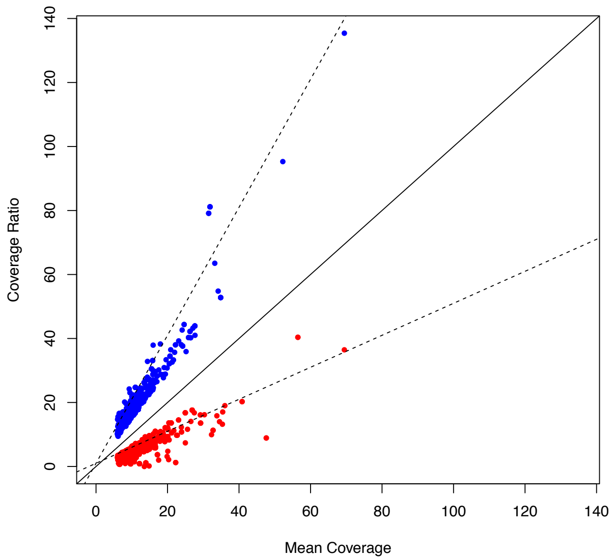
Supplemental Figure S1. The ratio of the mean depth of coverage between mutants and all other MA lines for duplications (blue) and deletions (red). The solid line indicates the 1:1 ratio as expected for non-CNVs, the dashed line indicates a 1:2 or 2:1 ratio representing a doubling or halving of copy number.
