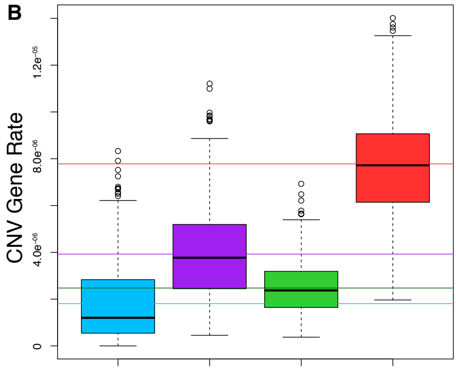
Supplemental Figure S2. CNV rates after permutation. CNV rates remain elevated in metal lines after using permutations to randomly sample (with replacement) 9 individuals from each treatment, with the mean indicated by a colored horizontal line. (A) CNV rates per nucleotide per generation and (B) complete gene CNV rates per single-copy gene per generation.
