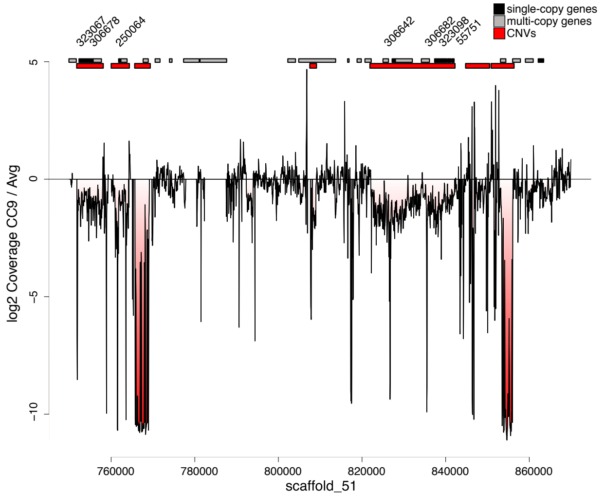
Supplemental Figure S6. Large deletion region in a non-MA isolate. The deletion encompasses seven single-copy genes, which are listed without the prefix “DAPPUDRAFT_”.
