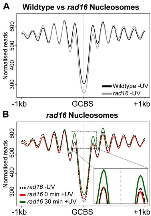
Figure S4 – Nucleosome occupancy and UV-induced chromatin remodeling at GCBS's is GG-NER dependent. A) Composite plots centred at GCBS positions are shown here depicting the nucleosome data from both wild type and RAD16 deleted GG-NER defective cells. B) As described in A, plotting MNase-seq data from RAD16 deleted GG-NER defective cells both before and after UV irradiation.
