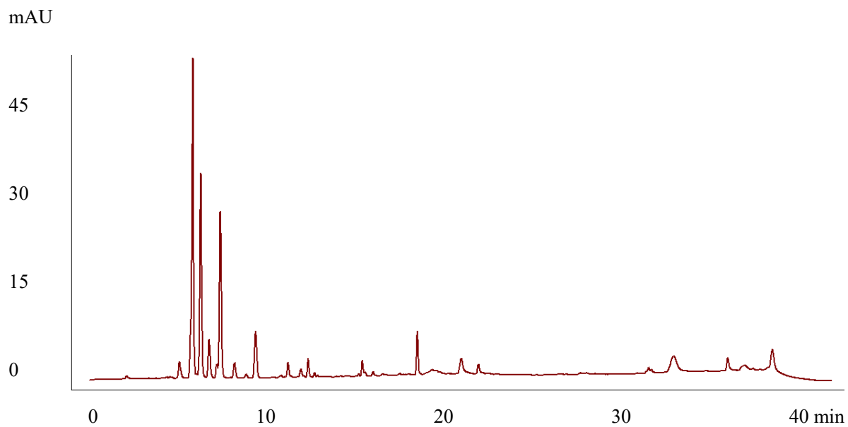
Figure S9. The HPLC fingerprints of collagen peptide sample S9
