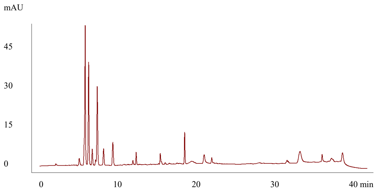
Figure S4. The HPLC fingerprints of collagen peptide sample S4
