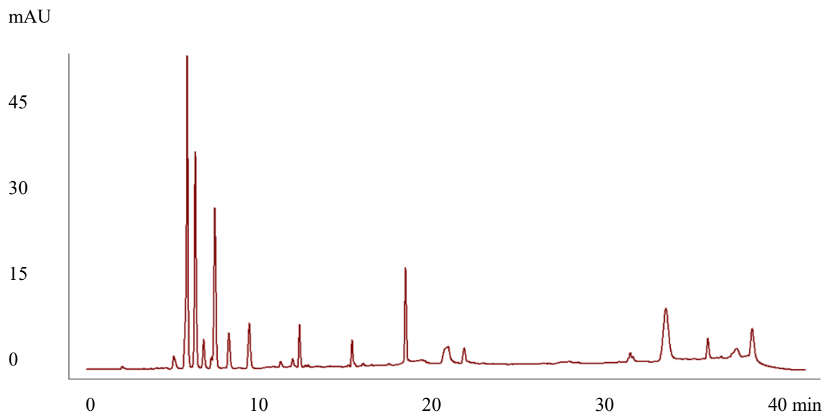
Figure S1. The HPLC fingerprints of collagen peptide sample S1
