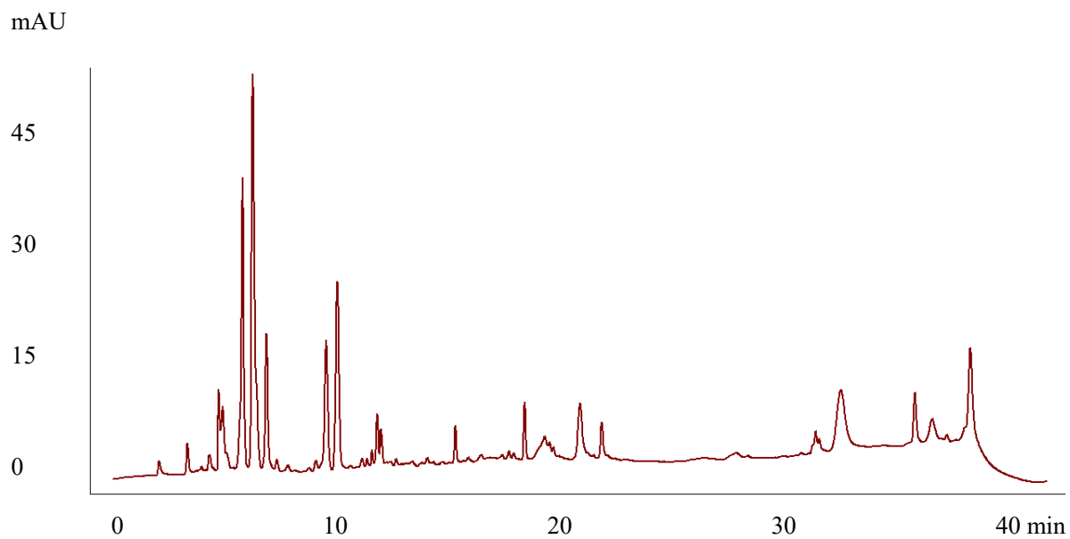
Figure S13. The HPLC fingerprints of collagen peptide sample S13
