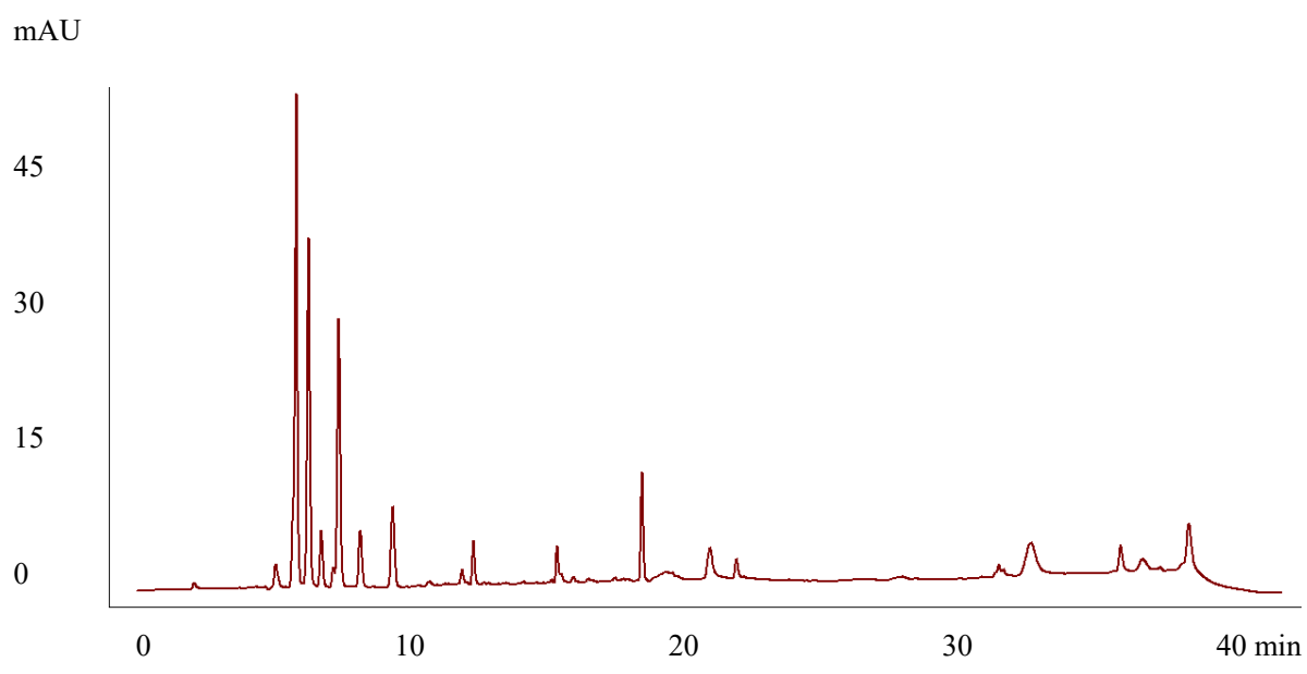
Figure S12. The HPLC fingerprints of collagen peptide sample S12
