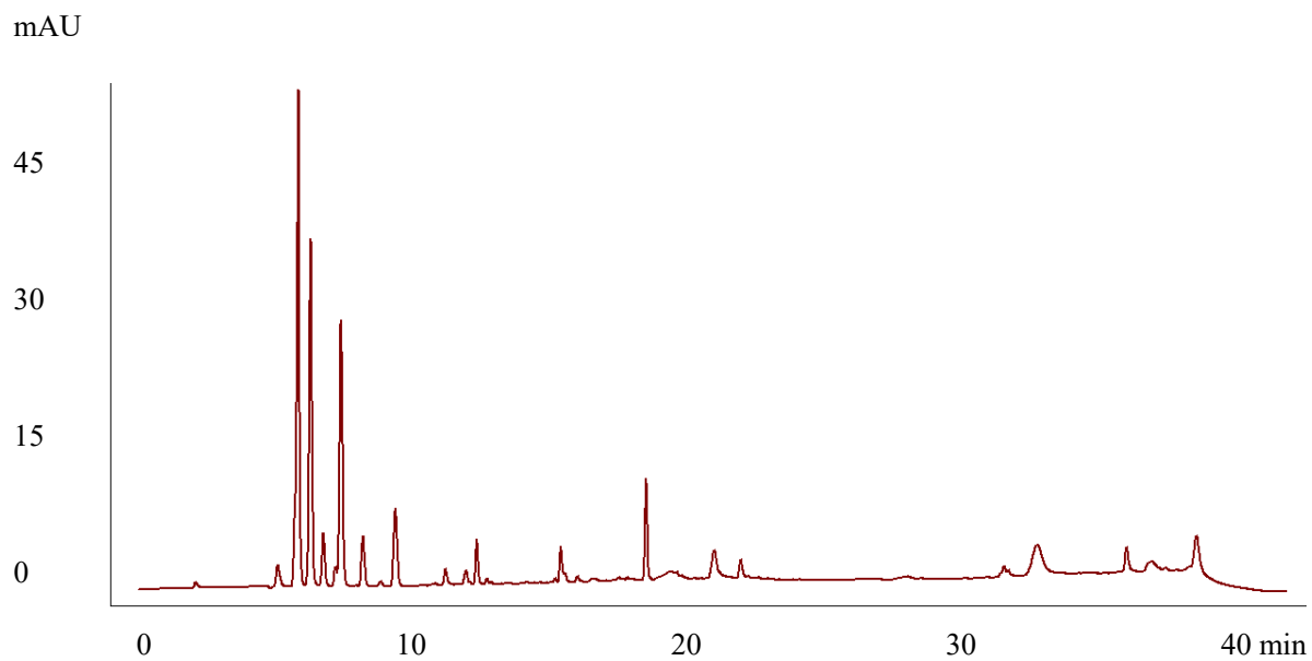
Figure S8. The HPLC fingerprints of collagen peptide sample S8
