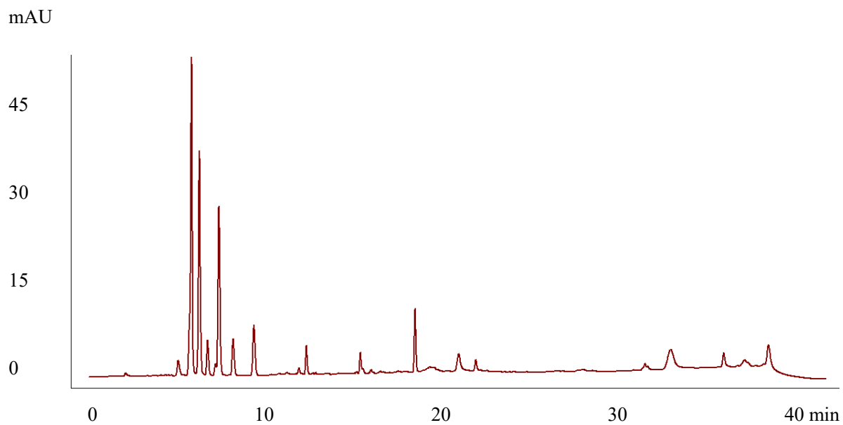
Figure S6. The HPLC fingerprints of collagen peptide sample S6
