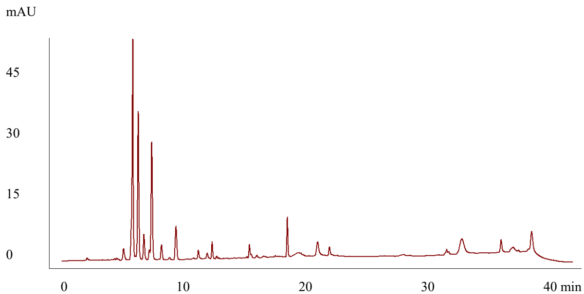
Figure S10. The HPLC fingerprints of collagen peptide sample S10
