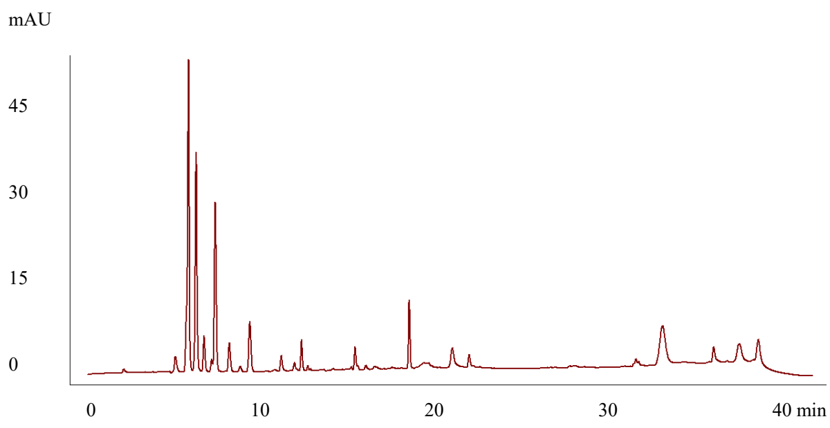
Figure S2. The HPLC fingerprints of collagen peptide sample S2
