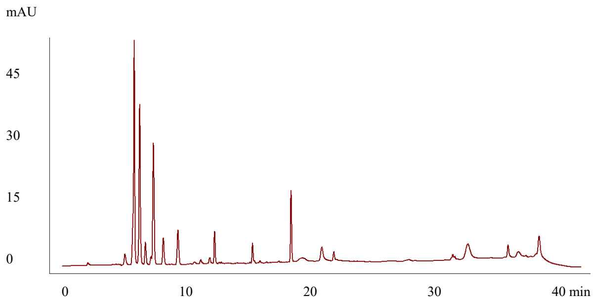
Figure S11. The HPLC fingerprints of collagen peptide sample S11
