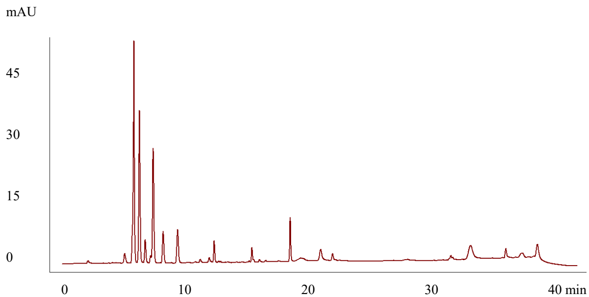
Figure S5. The HPLC fingerprints of collagen peptide sample S5
