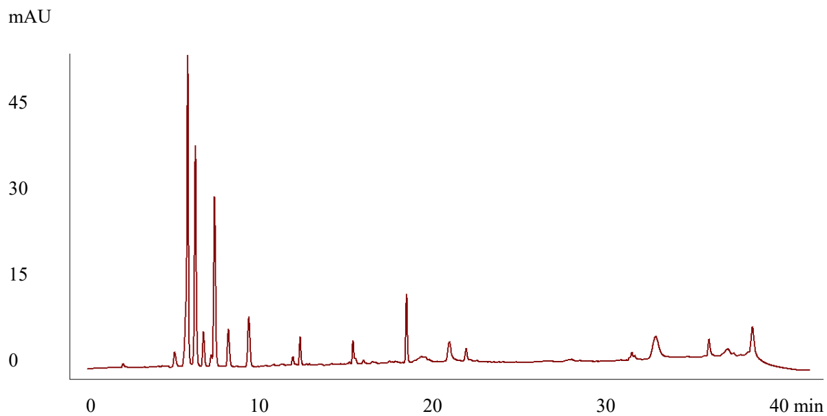
Figure S7. The HPLC fingerprints of collagen peptide sample S7
