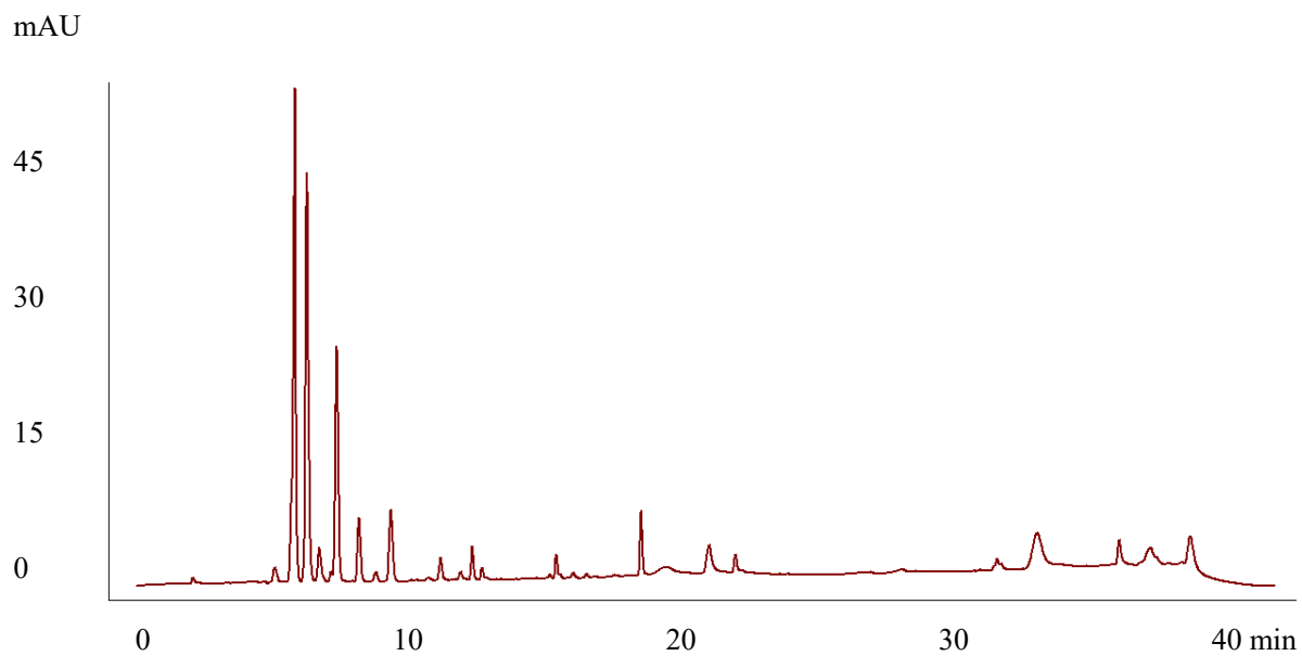
Figure S3. The HPLC fingerprints of collagen peptide sample S3
