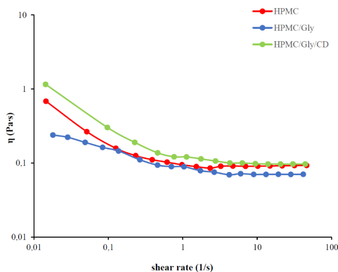
Figure S1. Flow curves of the film-forming solutions.
