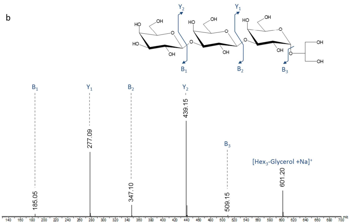
Supplementary data 1. ESI-MS/MS (+) spectra of the (hexose) 2 -glycerol ( a ) and the (hexose) 3 -glycerol ( b ) observed at m/z 439.15 and m/z 601.20 respectively.
