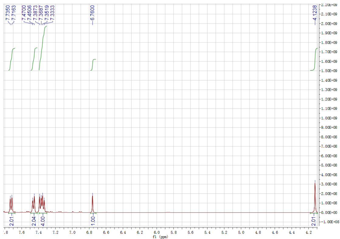
Figure S1. 1 H NMR spectrum of APCN
