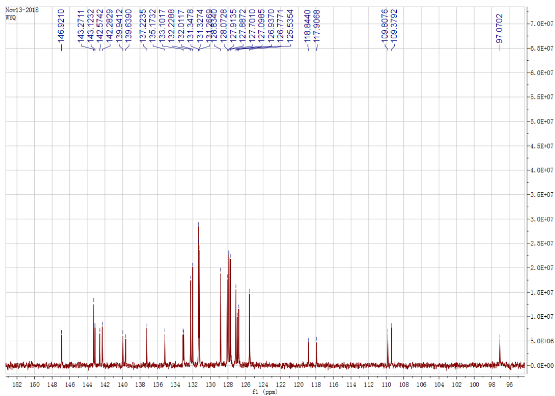
Figure S4. ^{13}\text{C} NMR spectrum of APPTPECN
