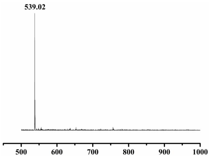
Figure S2. MALDI-TOF spectrum of APCN
