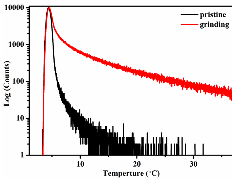
Figure S7. Fluorescence decay curves for solid-state of APPTPECN before and after grinding
