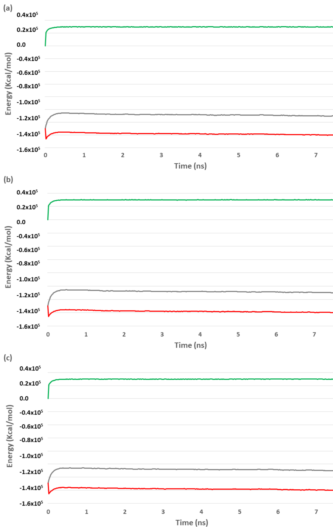
Figure S3. MD simulation: Energy profile for the (a) TAK-285, (b) 1a, (c) 1d. total energy (grey color), potential energy (red color), kinetic energy (green color)
