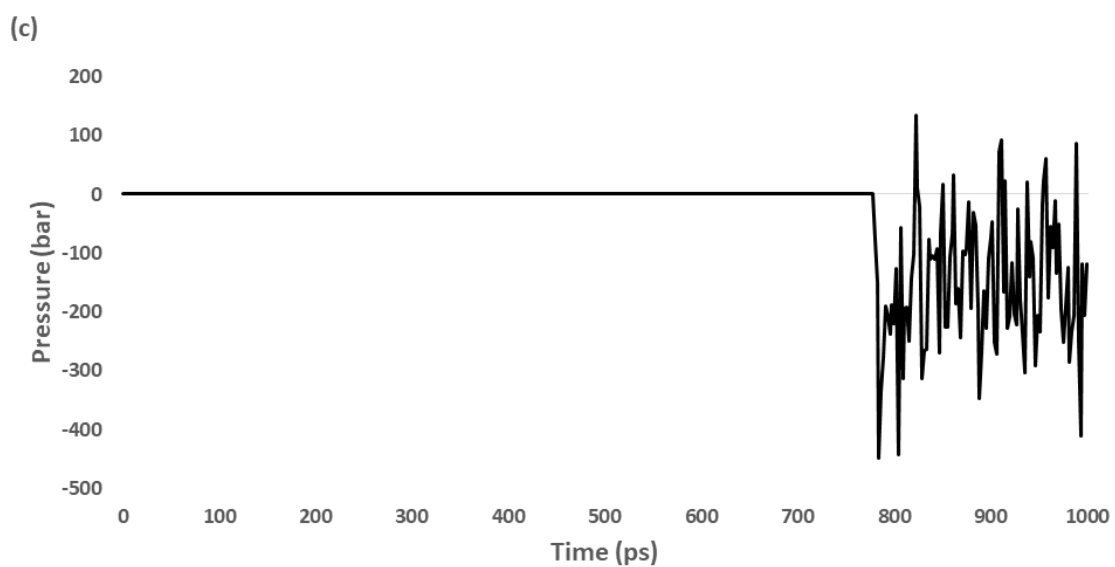
Figure S2: MD simulation: pressure profile during equilibration for the (a) TAK-285, (b) 1a, (c) 1d.
