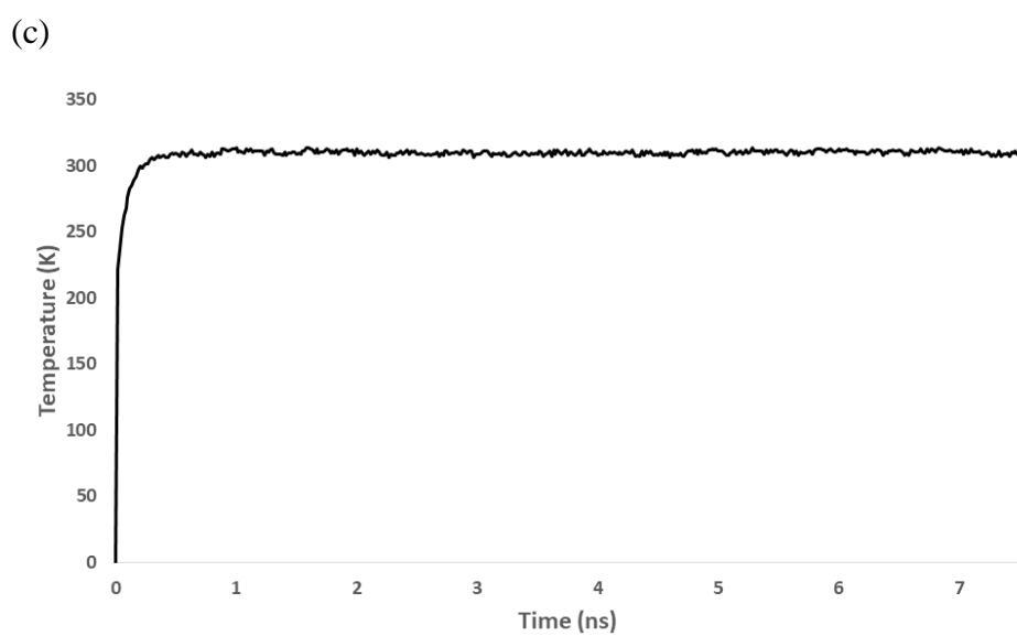
Figure S1: MD simulation: Temperature profile during 7 ns for the (a) TAK-285 , (b) 1a , (c) 1d .
