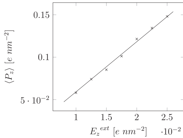
Figure S1: Averaged polarization response of our polarizable water model ( \langle P_z \rangle ) to an external electric field ( E_z^{ext} ), used to determine the model's static dielectric permittivity by linear regression ( R^2 > 0.99 ).
