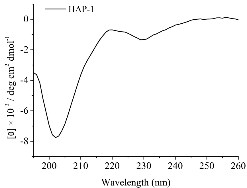
Figure S1. Far-UV CD spectrum of HAP-1. The concentration of the peptide was 1.0 mg/mL. Temperature was 25 °C.
