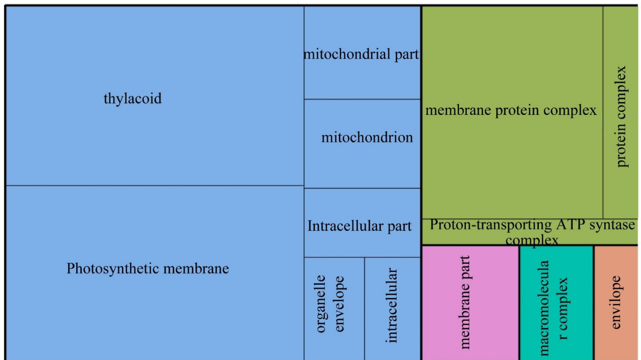
Figure S4. TreeMap showing GO enrichment analysis results for all protein precursors for cell peptides.
