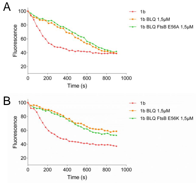
Figure S3. Effect of FtsBLQ containing FtsB mutations E56A (A) or E56K (B) on the GTase activity of PBP1b measured by continuous fluorescence assay.
