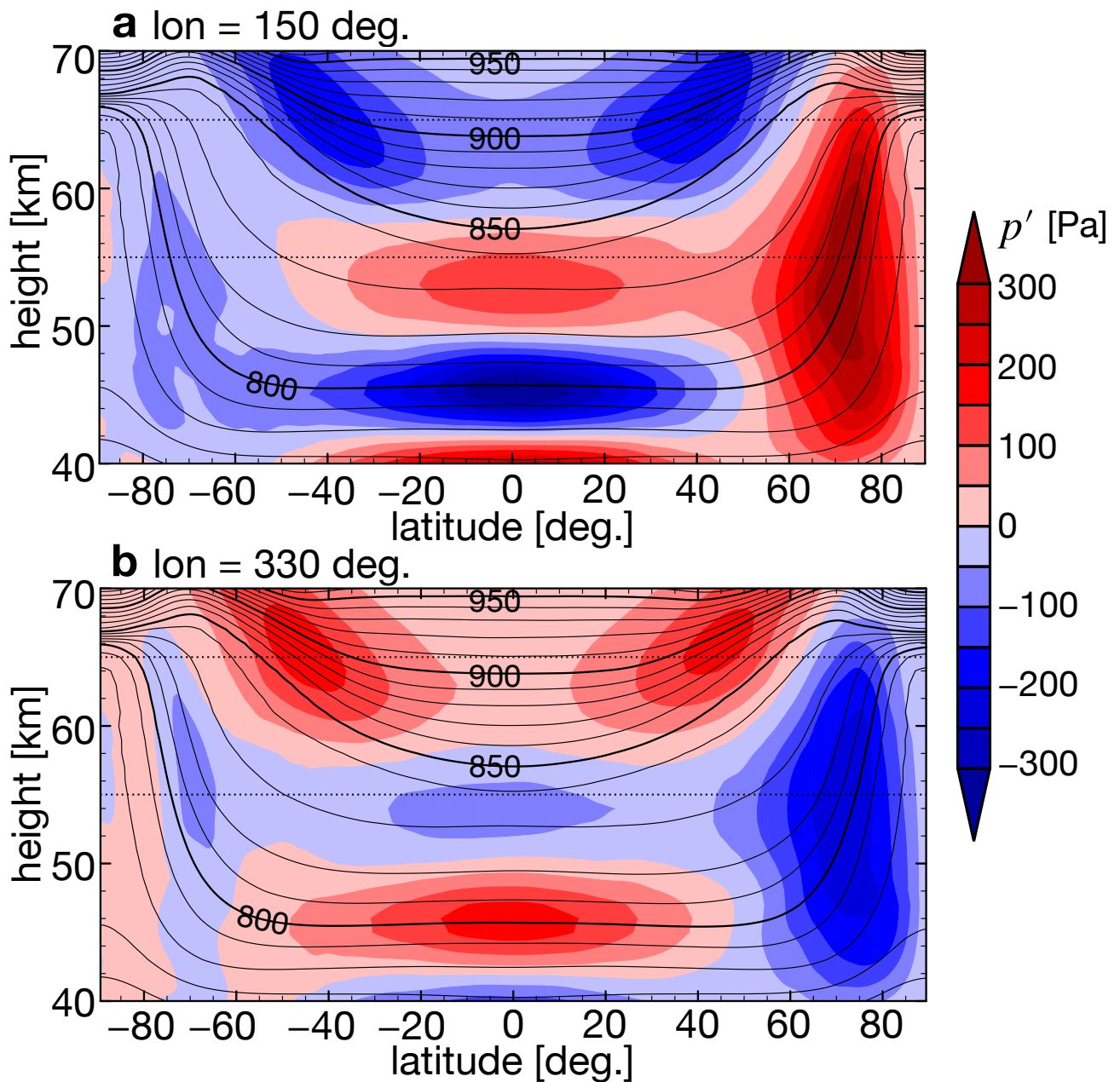
Supplementary Figure 1: Latitude-height cross-sections of the pressure anomaly (colour) in the composite mean of the ZS0 case. Longitudes are (a) 150 deg. and (b) 330 deg. Contours indicate the zonally and temporally averaged potential temperature that is the same as Fig. 5f. The contour interval is 10 K. Horizontal dotted lines show heights of 55 km and 65 km.
