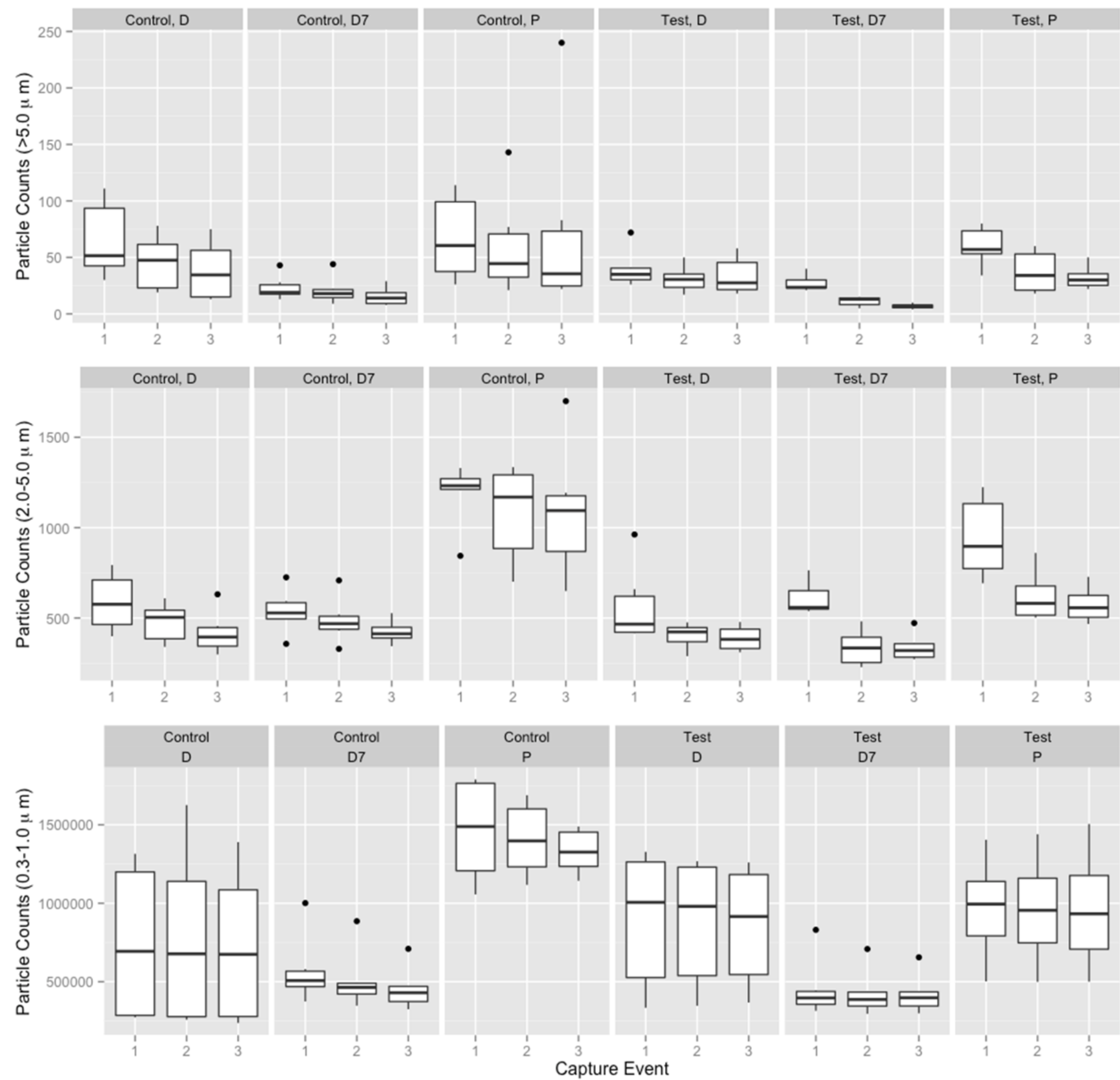
Supplemental Figure S1: Particle Counts (measured with MetOne GT-526) across Control (without faucet) and Test (with faucet) experiments of D-Drain inoculation, D7-Drainline colonization and P-P-trap inoculation methods.
