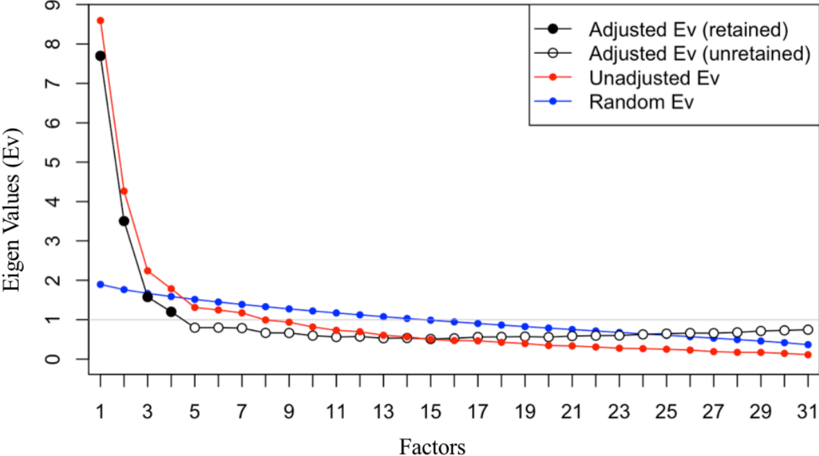
Scree Plot of Eigen Values and Factors Retained
