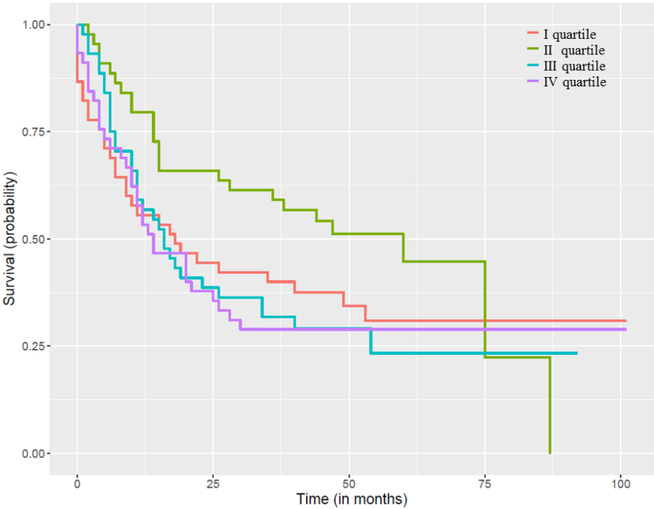
S3 Fig. Kaplan-Meier curves of 8-years survival depending on UIBC
