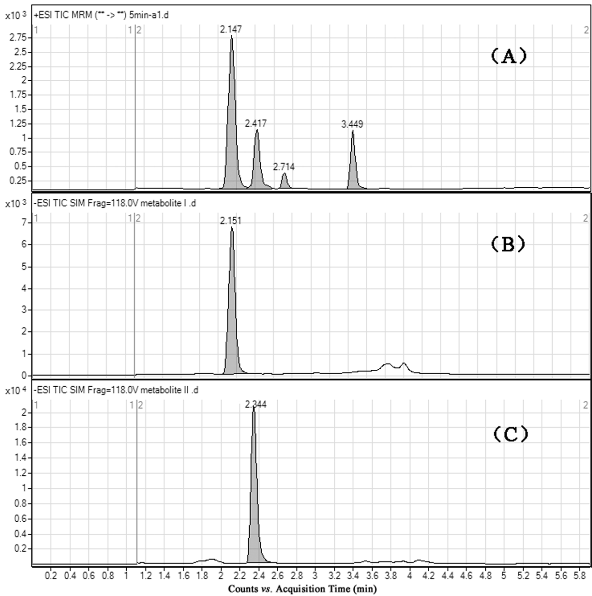
Figure S1. Representative chromatograms of scopoletin/metabolites in rat plasma: (A) MRM chromatogram of scopoletin and IS; (B) SIM chromatogram of scopoletin-glucuronide conjugate; (C) SIM chromatogram of scopoletin-sulfate conjugate.
