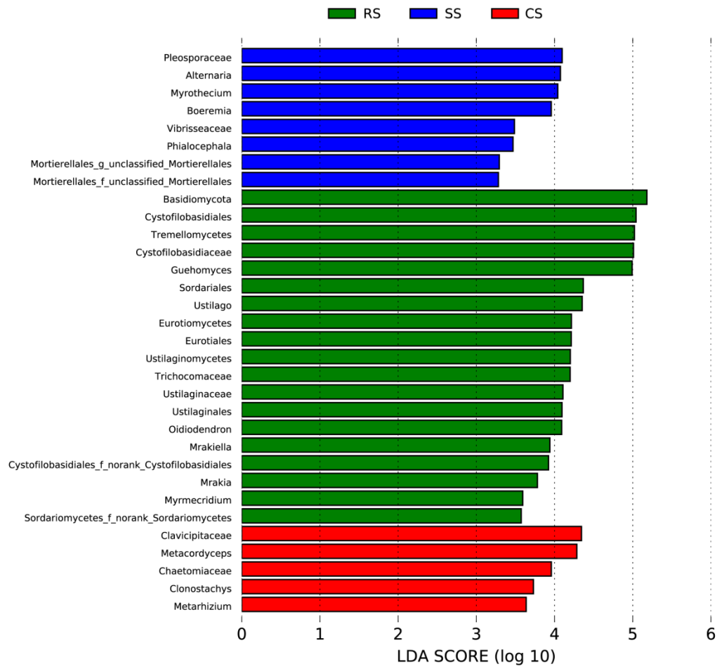
Figure S1 | Histogram of the linear discriminant analysis (LDA) scores. Taxa enriched in CS are shown in red with a positive LDA score, RS in green with positive LDA score and SS in blue with a positive LDA score ( P < 0.05 ; LDA score 2.0).
