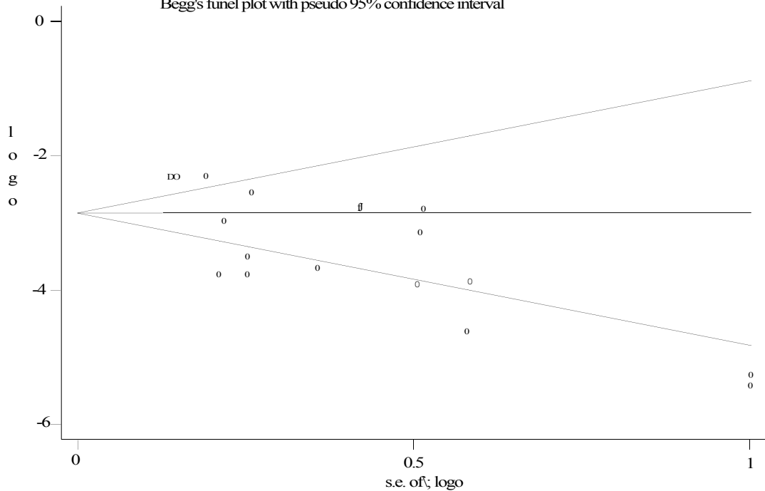
Begg's funnel plot with pseudo 95% confidence interval
