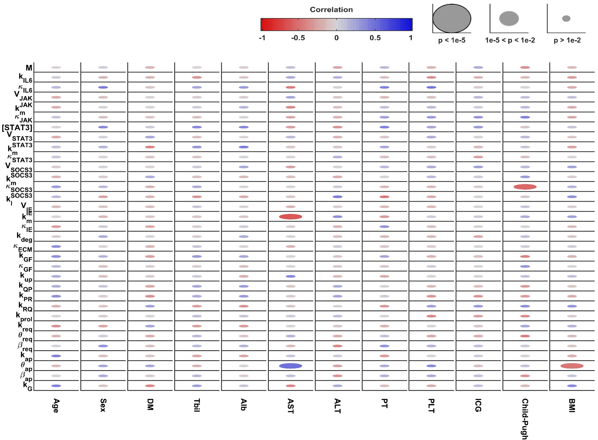
Figure S2: Pairwise correlation between optimized model parameters with clinical data of the 27 patients from Yamamoto et al. [18]. There is no significant pairwise correlation between parameters and the available clinical information (Bonferroni corrected p-value < 1e-5 ).
