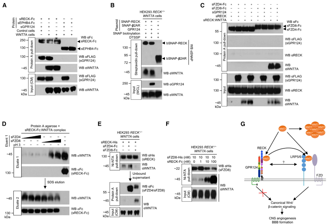
Figure 4. RECK Promotes FZD8:WNT7A Complex Formation
