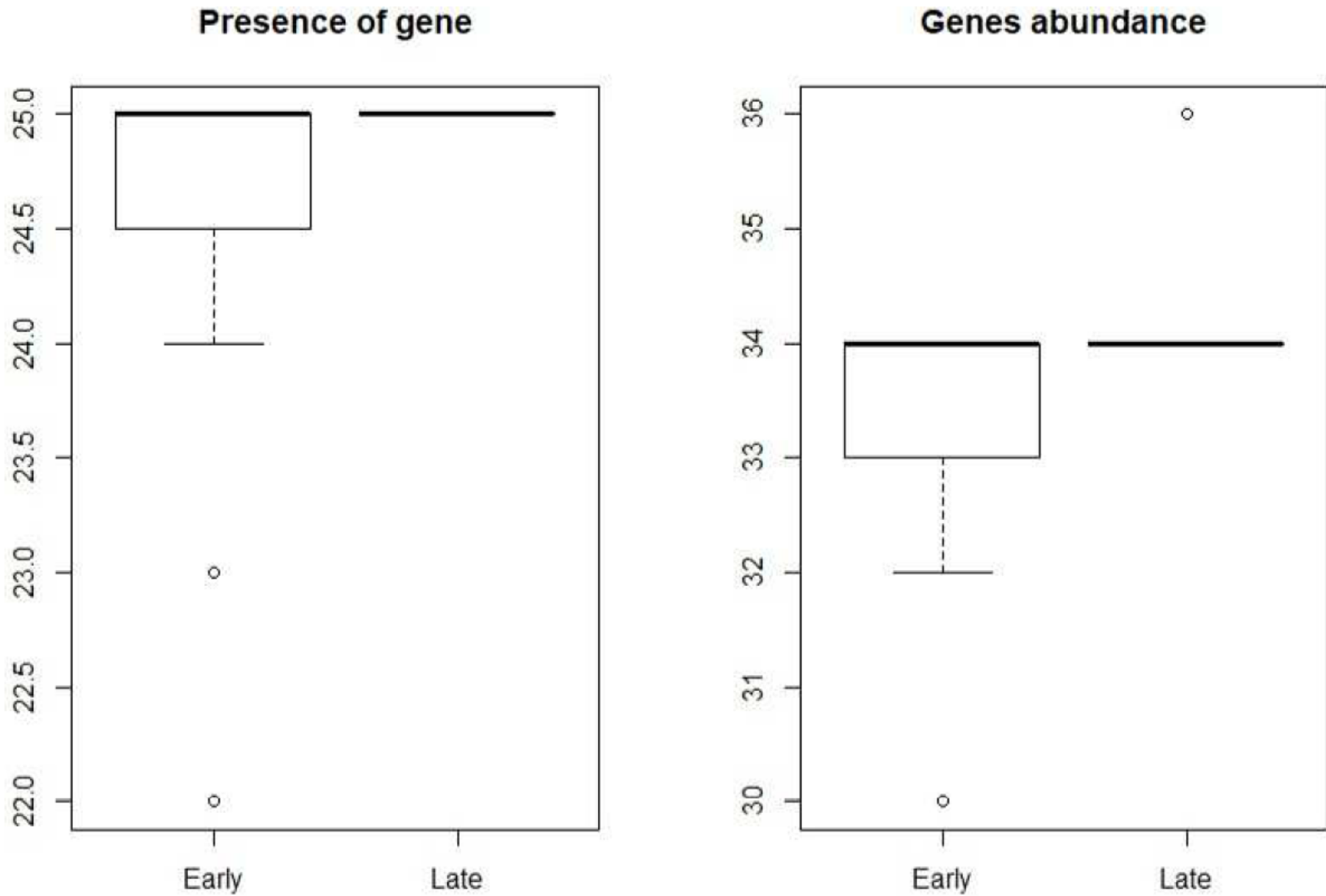
Additional file 10: Figure S8: Boxplots of TA genes.
