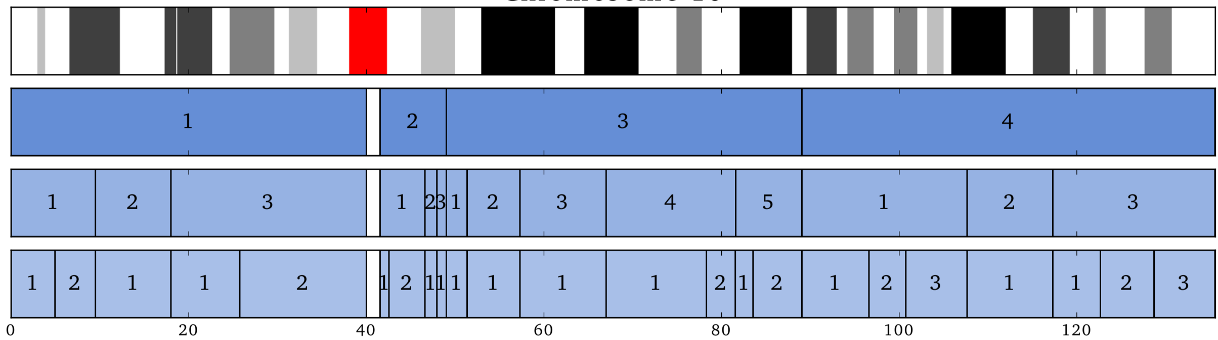
Chromosome 11
