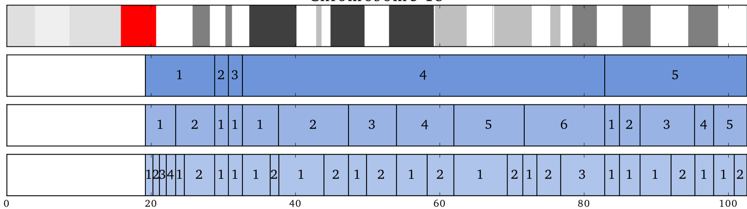
Chromosome 16
