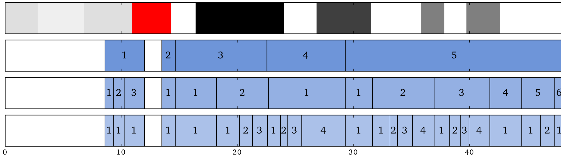
Chromosome 22
