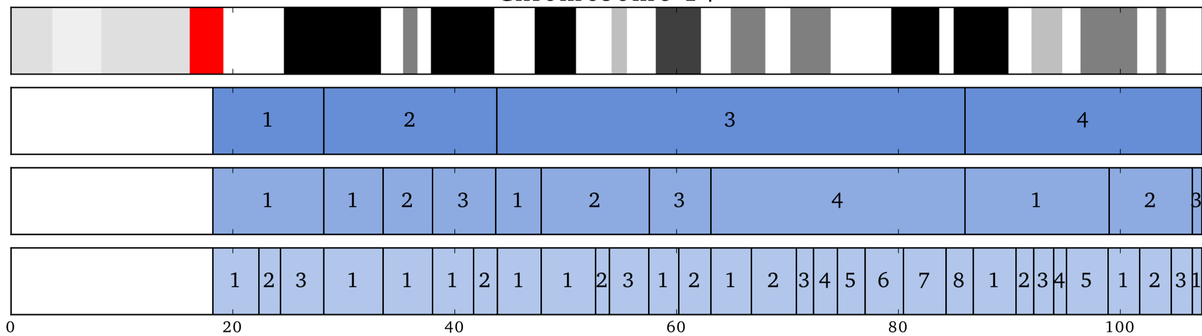
Chromosome 15
