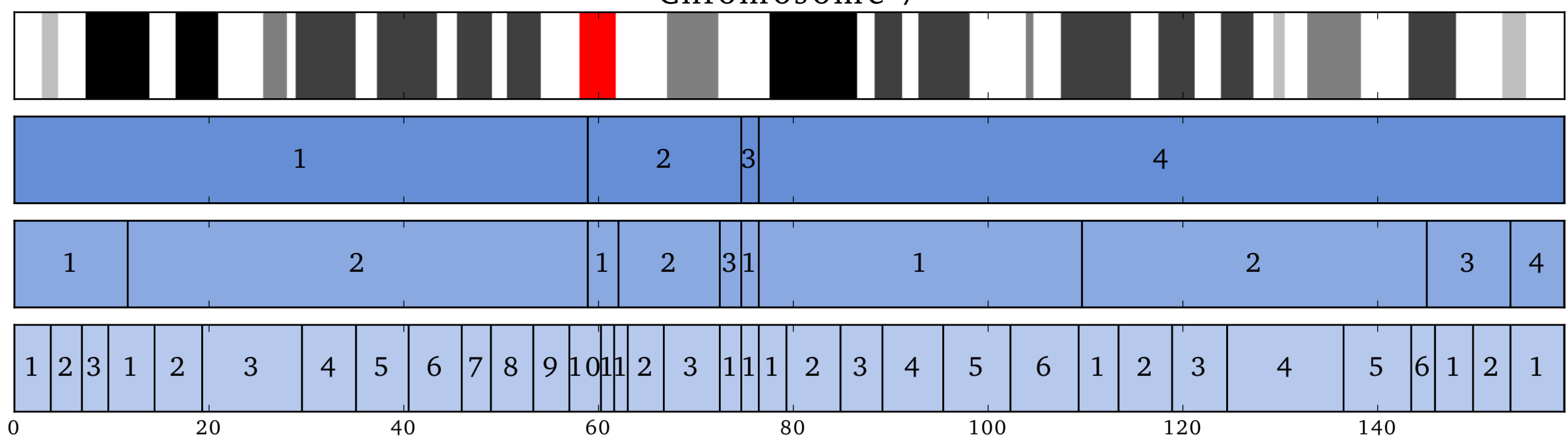
Chromosome 8
