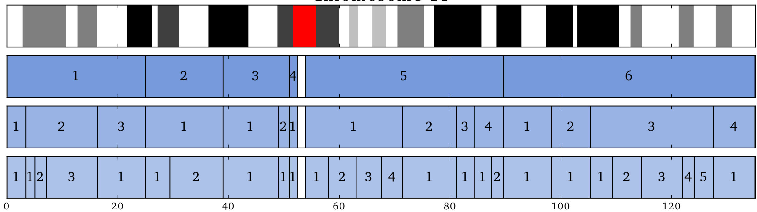
Chromosome 12
