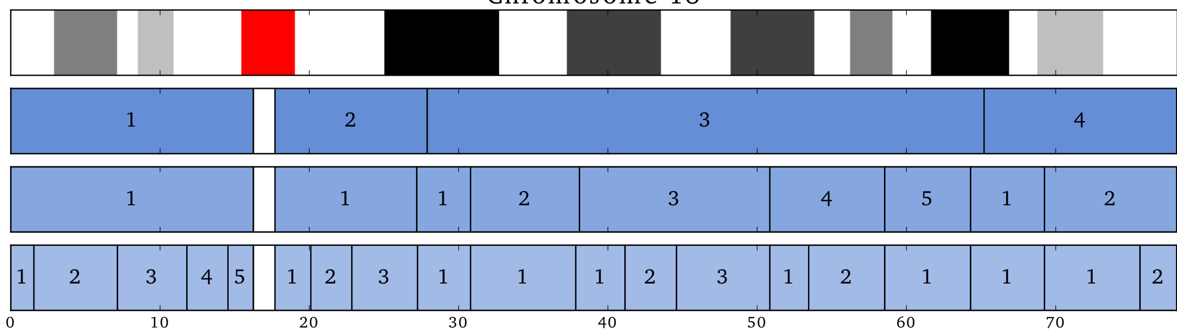
Chromosome 18
