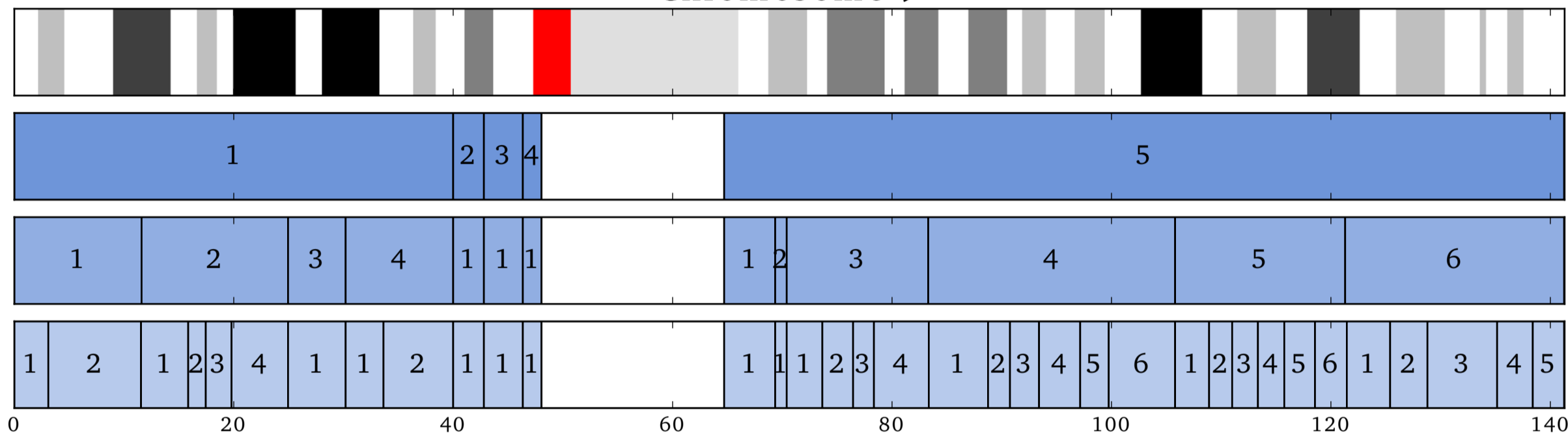
Chromosome 10
