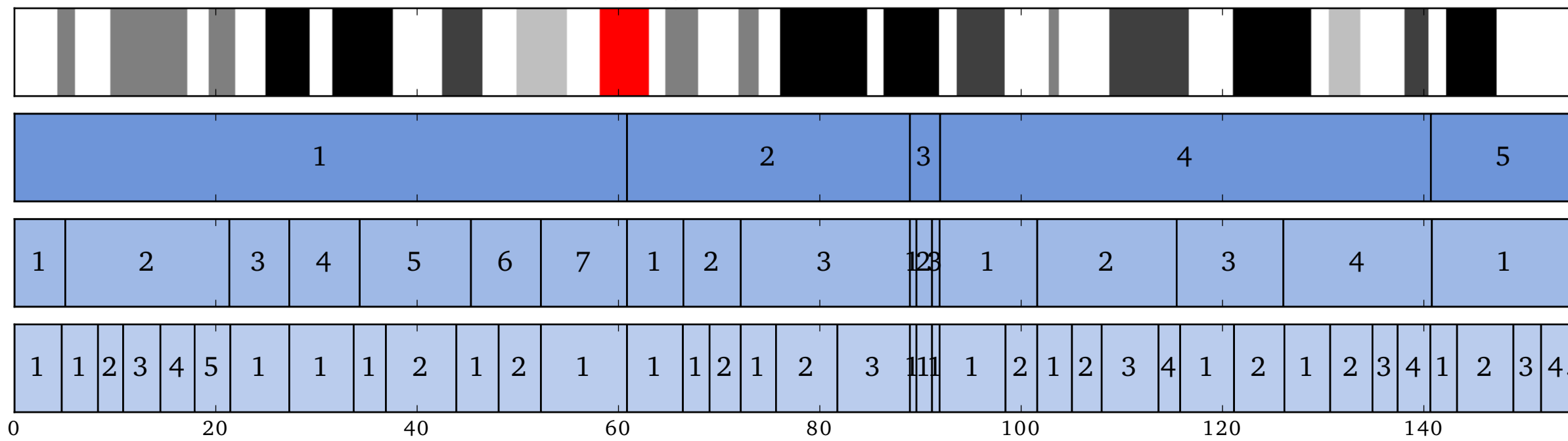
Chromosome X
