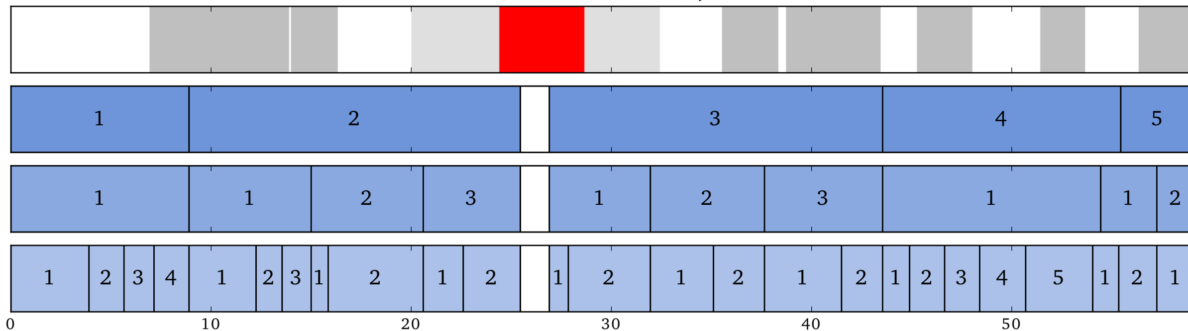
Chromosome 20
