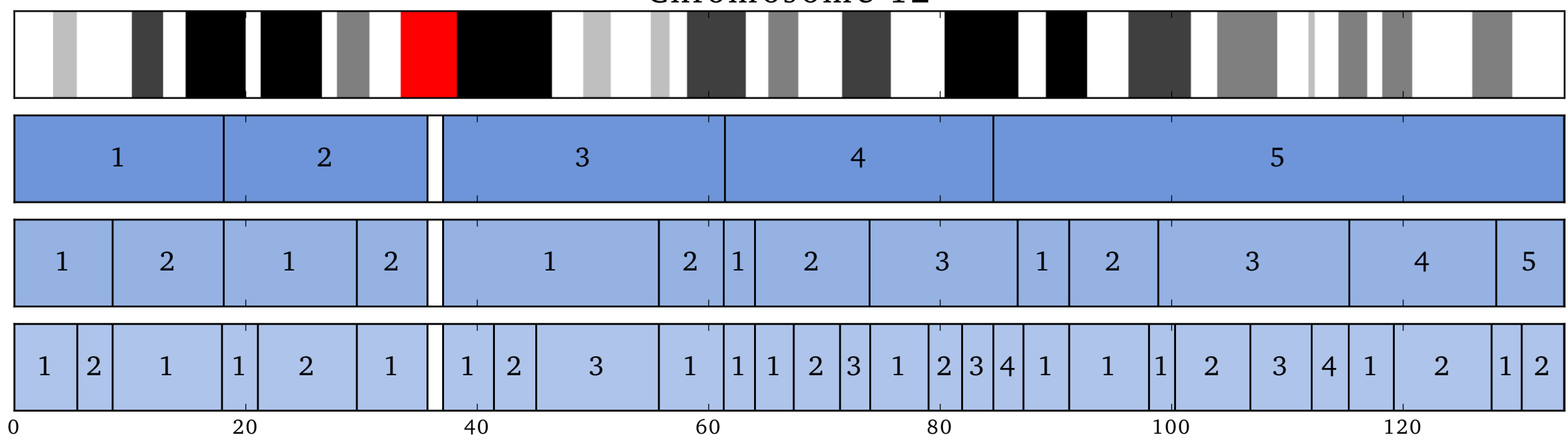
Chromosome 12
