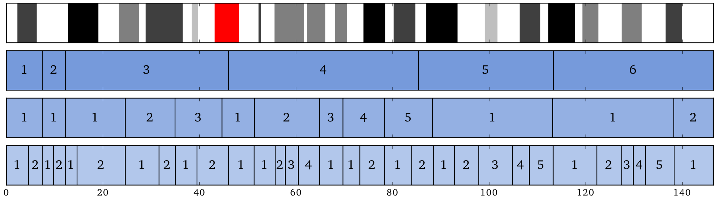
Chromosome 9
