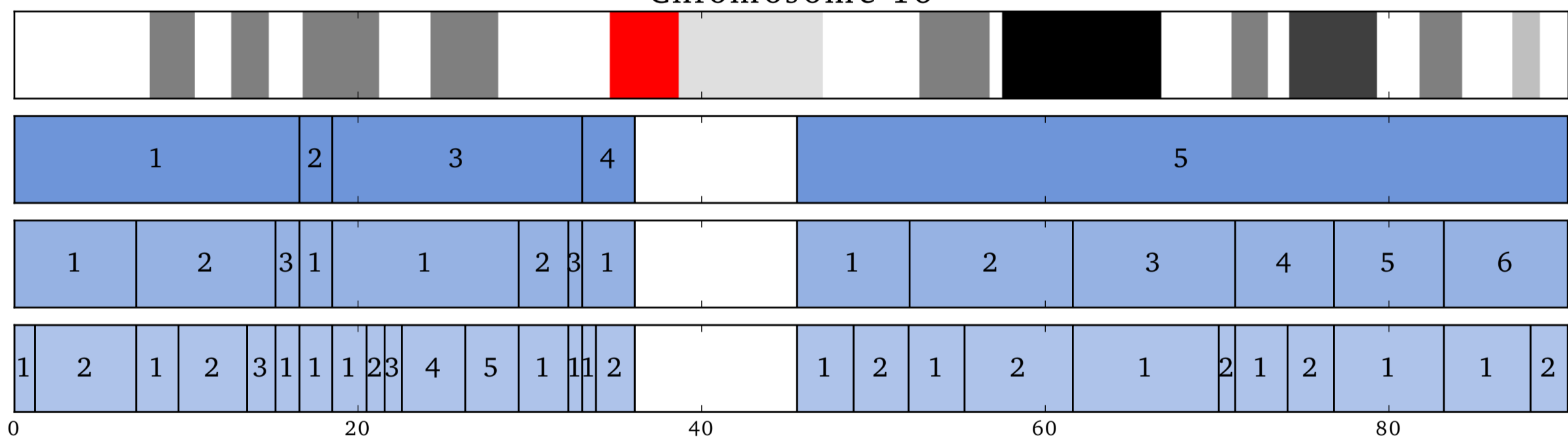
Chromosome 17
