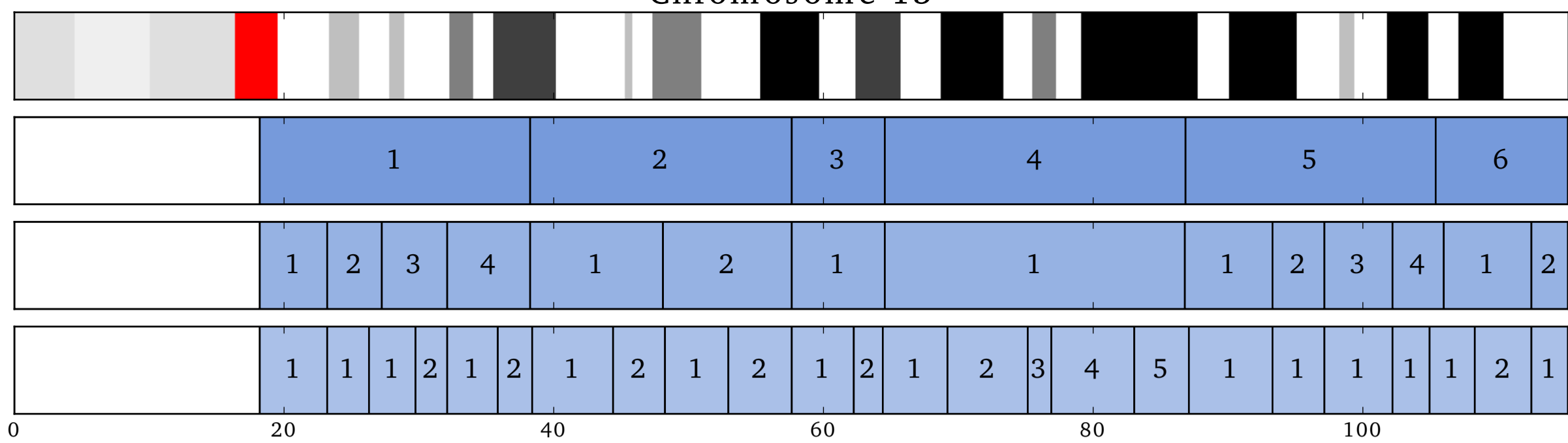
Chromosome 14
