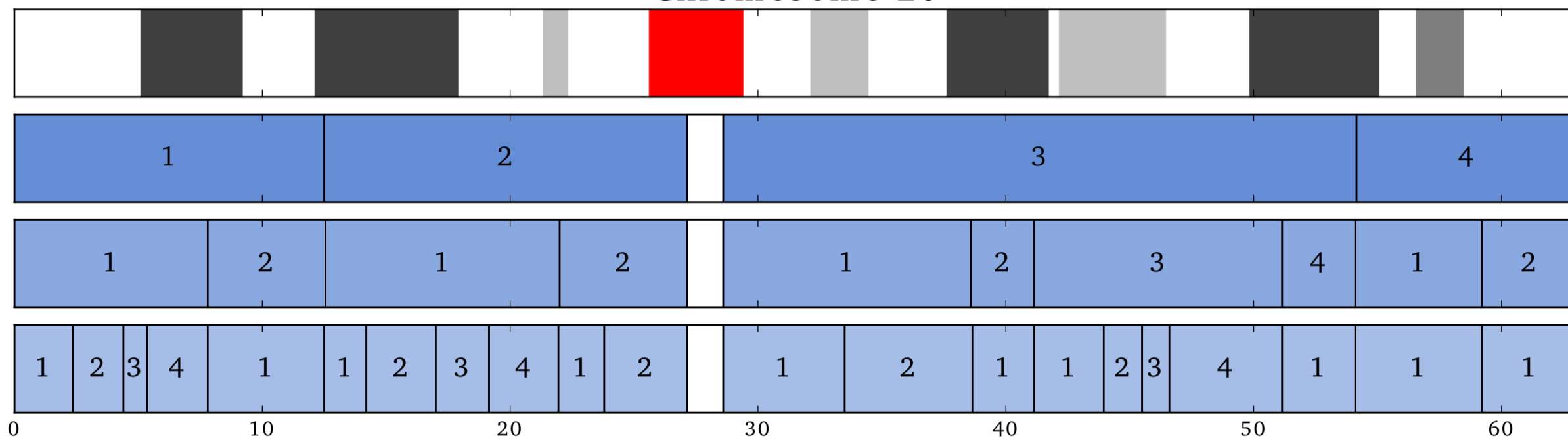
Chromosome 21
