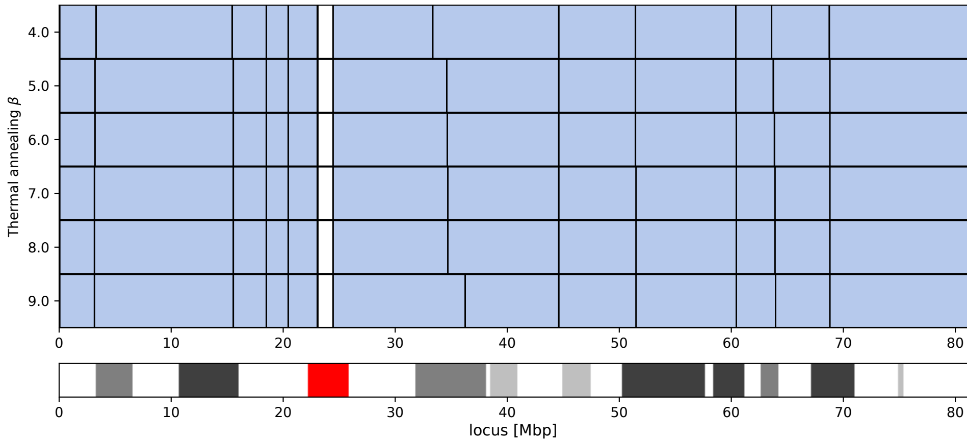
Partitioning of chromosome 17 with varying \beta
