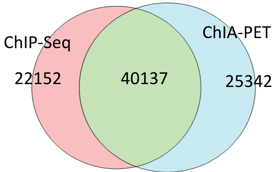
Figure.S1: Venn diagram shows the overlapping the fraction between ARBS defined by ChIP-seq experiment and ChIA-PET experiment.
