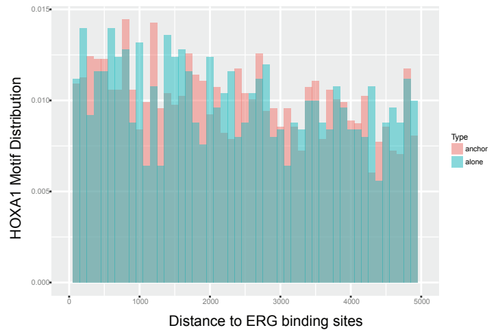
Figure S10: Upper panel: FOXA1 motif distance distribution to AR (ERG) binding sites with chromatin looping (red) and without chromatin looping (green). FOXA1 motif shows strongly enriched to AR and ERG binding site regardless with/without looping. Bottom panel: HOXA1 motif distance distribution to AR (ERG) binding sites with chromatin looping (red) and without chromatin looping (green). HOXA1 motif doesn't show strong enrichment to AR and ERG binding site regardless with/without looping.
