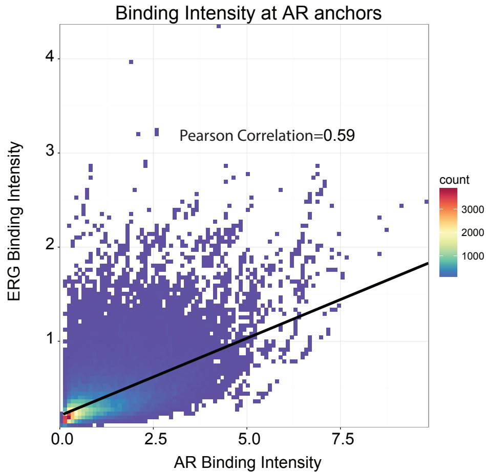
Figure.S11: Binding intensity of AR and ERG on AR ChIA-PET interaction anchor. The binding intensity is the average read depth from our ChIP-seq data of AR and ERG (2hour after DHT). The solid black line represent the linear regression line, and the pearson correlation of the binding intensity between AR and ERG is 0.59 .
