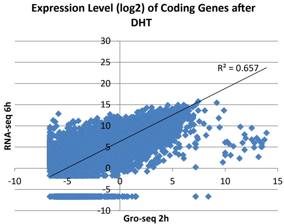
Figure.S9: Correlation between Gro-Seq and RNA-seq. (a)- Gro-seq 0h vs RNA-seq 0h. (b) Gro-seq 2h vs RNA-seq 6h
