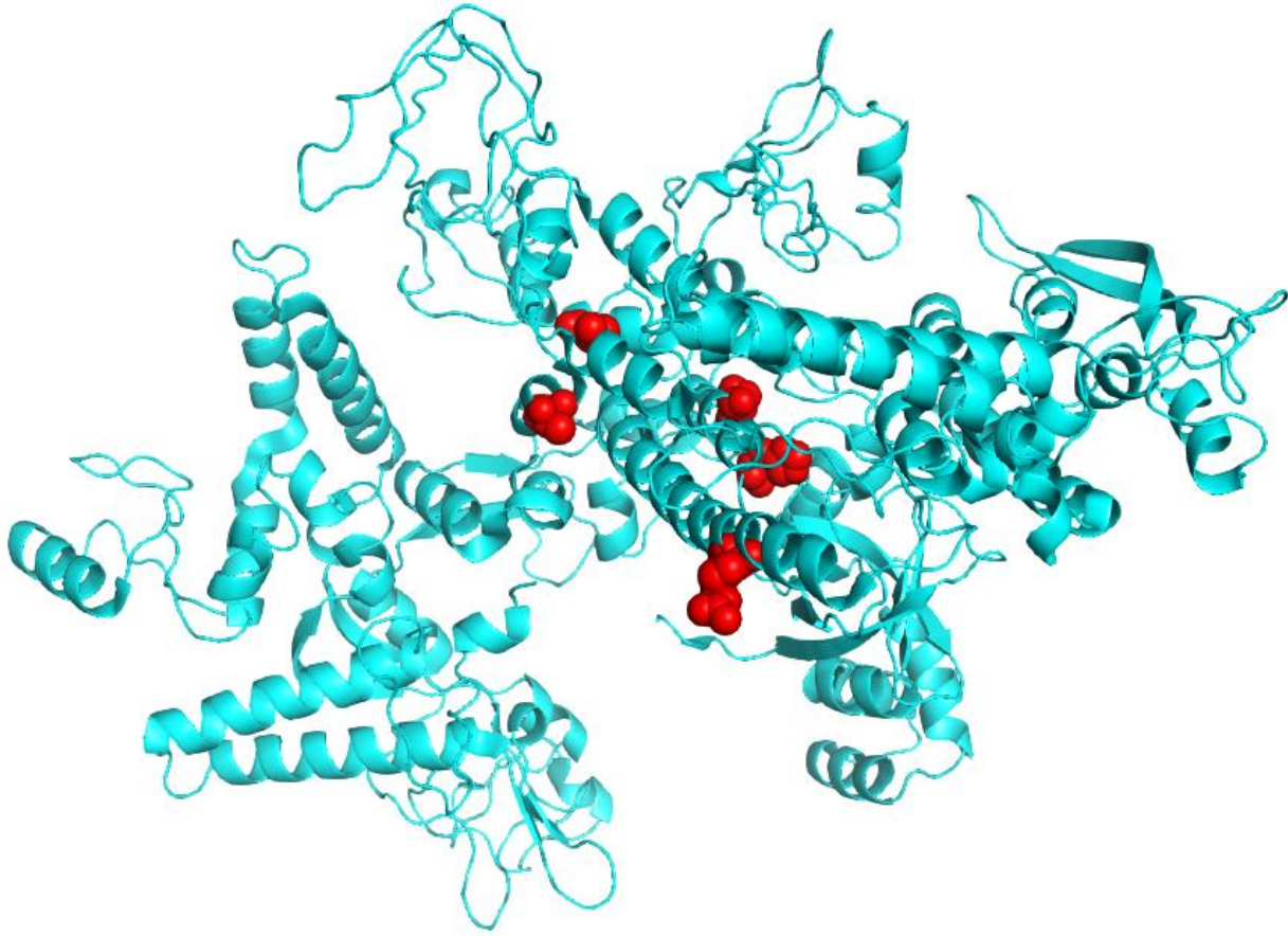
Figure S1. Structural representation of RpoC with the positions of the mutations highlighted in red.
